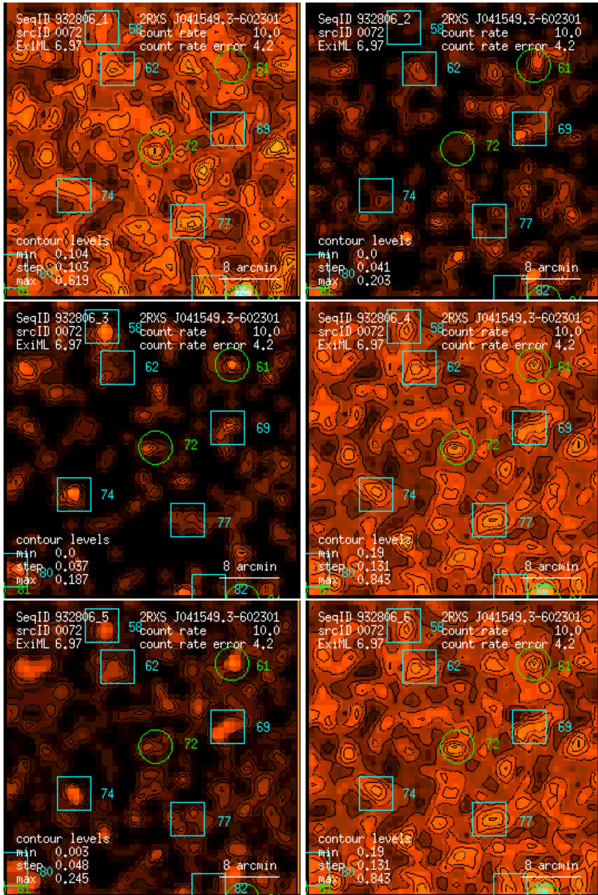
Figure 72: RASS 932806: detection 0072: band rate images, Gaussian filter: (1) PSPC channels 11 – 41, (2) 52 – 90, (3) 91 – 201, (4) 11 – 235, (5) 52 – 201, (6) 11 – 201. Broad band rates in counts/ks. Band rate contour levels in counts/ks/arcmin 2 .
