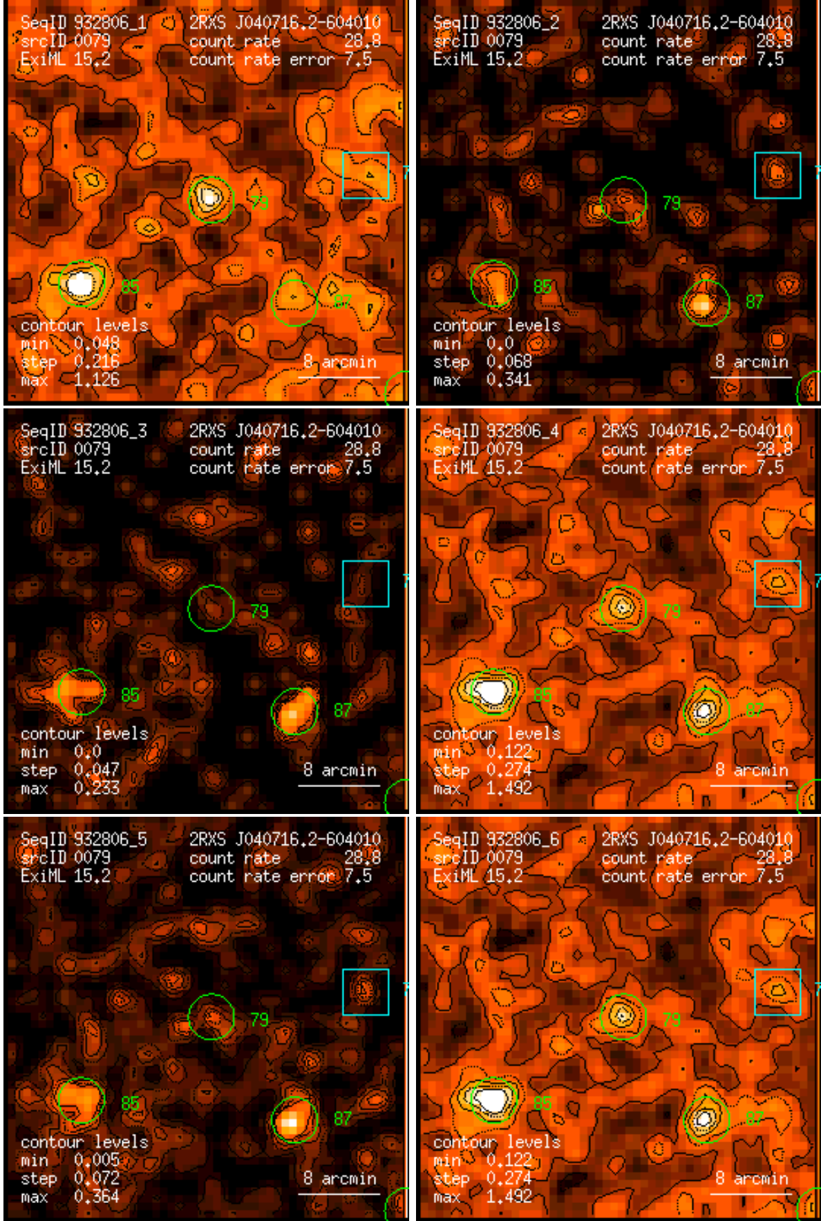
Figure 79: RASS 932806: detection 0079: band rate images, Gaussian filter: (1) PSPC channels 11 – 41, (2) 52 – 90, (3) 91 – 201, (4) 11 – 235, (5) 52 – 201, (6) 11 – 201. Broad band rates in counts/ks. Band rate contour levels in counts/ks/arcmin 2 .
