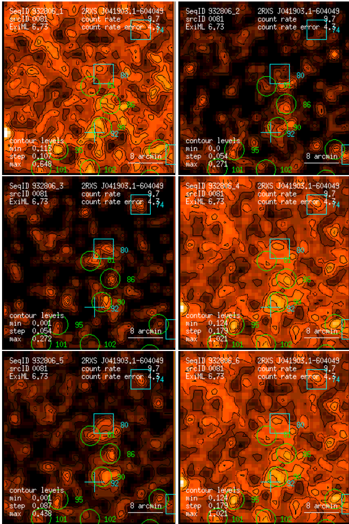
Figure 81: RASS 932806: detection 0081: band rate images, Gaussian filter: (1) PSPC channels 11 – 41, (2) 52 – 90, (3) 91 – 201, (4) 11 – 235, (5) 52 – 201, (6) 11 – 201. Broad band rates in counts/ks. Band rate contour levels in counts/ks/arcmin 2 .
