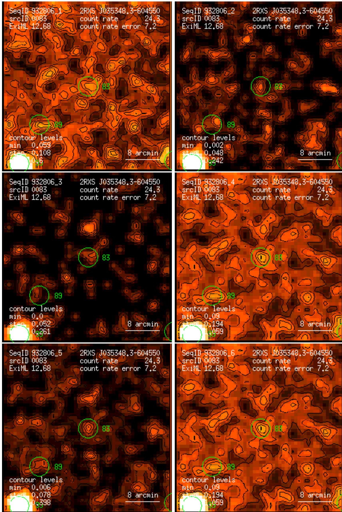
Figure 83: RASS 932806: detection 0083: band rate images, Gaussian filter: (1) PSPC channels 11 – 41, (2) 52 – 90, (3) 91 – 201, (4) 11 – 235, (5) 52 – 201, (6) 11 – 201. Broad band rates in counts/ks. Band rate contour levels in counts/ks/arcmin 2 .
