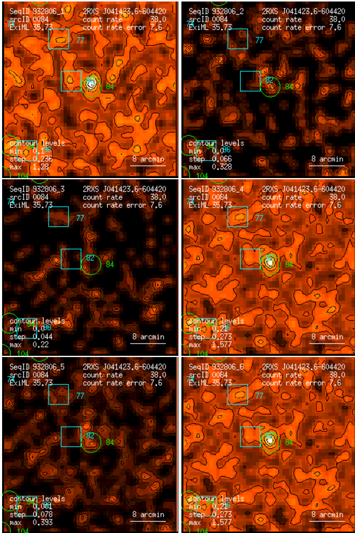
Figure 84: RASS 932806: detection 0084: band rate images, Gaussian filter: (1) PSPC channels 11 – 41, (2) 52 – 90, (3) 91 – 201, (4) 11 – 235, (5) 52 – 201, (6) 11 – 201. Broad band rates in counts/ks. Band rate contour levels in counts/ks/arcmin 2 .
