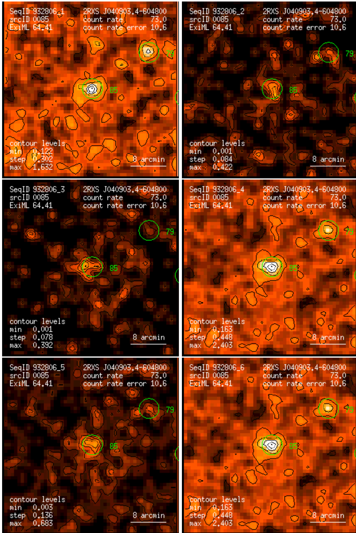
Figure 85: RASS 932806: detection 0085: band rate images, Gaussian filter: (1) PSPC channels 11 – 41, (2) 52 – 90, (3) 91 – 201, (4) 11 – 235, (5) 52 – 201, (6) 11 – 201. Broad band rates in counts/ks. Band rate contour levels in counts/ks/arcmin 2 .
