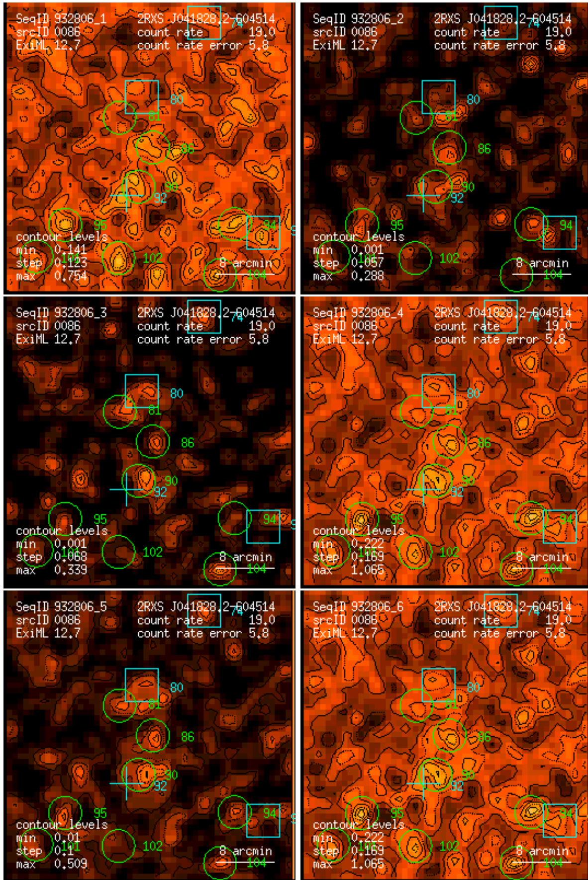
Figure 86: RASS 932806: detection 0086: band rate images, Gaussian filter: (1) PSPC channels 11 – 41, (2) 52 – 90, (3) 91 – 201, (4) 11 – 235, (5) 52 – 201, (6) 11 – 201. Broad band rates in counts/ks. Band rate contour levels in counts/ks/arcmin 2 .
