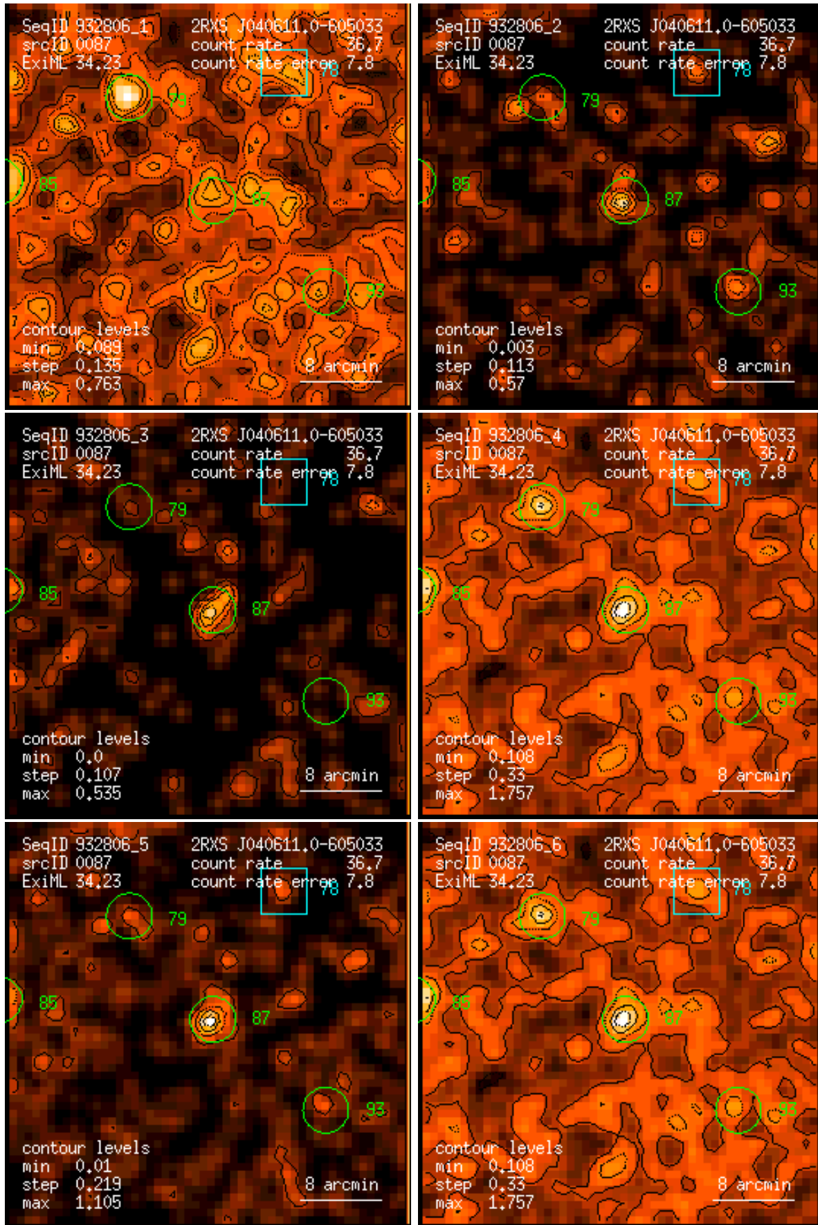
Figure 87: RASS 932806: detection 0087: band rate images, Gaussian filter: (1) PSPC channels 11 – 41, (2) 52 – 90, (3) 91 – 201, (4) 11 – 235, (5) 52 – 201, (6) 11 – 201. Broad band rates in counts/ks. Band rate contour levels in counts/ks/arcmin 2 .
