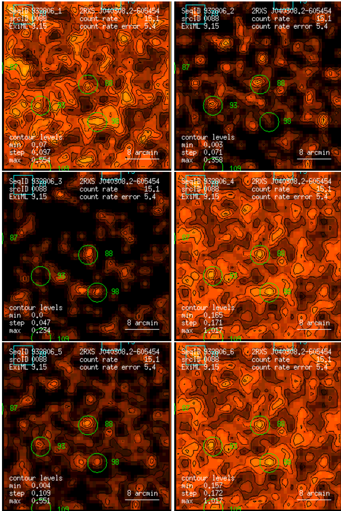
Figure 88: RASS 932806: detection 0088: band rate images, Gaussian filter: (1) PSPC channels 11 – 41, (2) 52 – 90, (3) 91 – 201, (4) 11 – 235, (5) 52 – 201, (6) 11 – 201. Broad band rates in counts/ks. Band rate contour levels in counts/ks/arcmin 2 .
