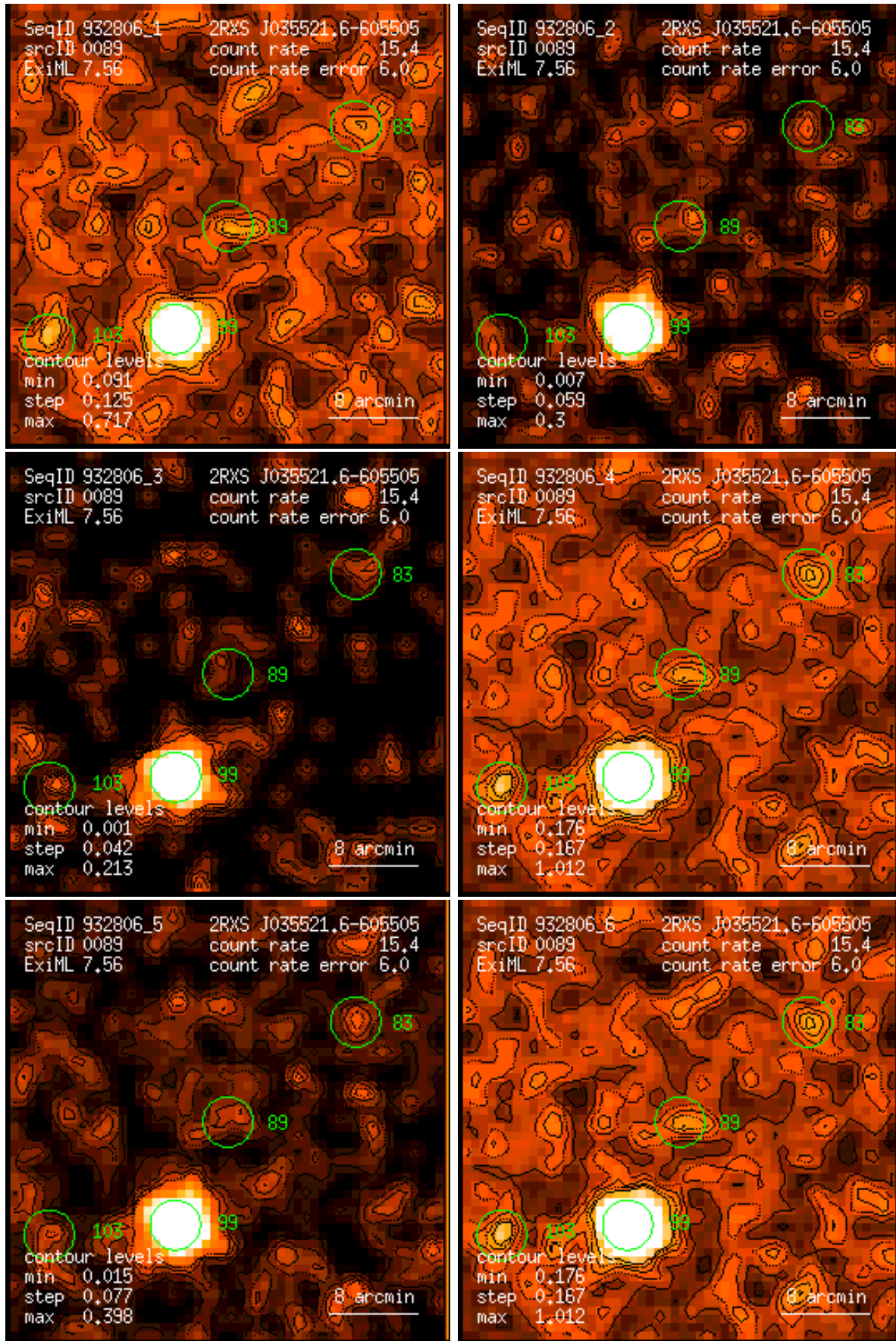
Figure 89: RASS 932806: detection 0089: band rate images, Gaussian filter: (1) PSPC channels 11 – 41, (2) 52 – 90, (3) 91 – 201, (4) 11 – 235, (5) 52 – 201, (6) 11 – 201. Broad band rates in counts/ks. Band rate contour levels in counts/ks/arcmin 2 .
