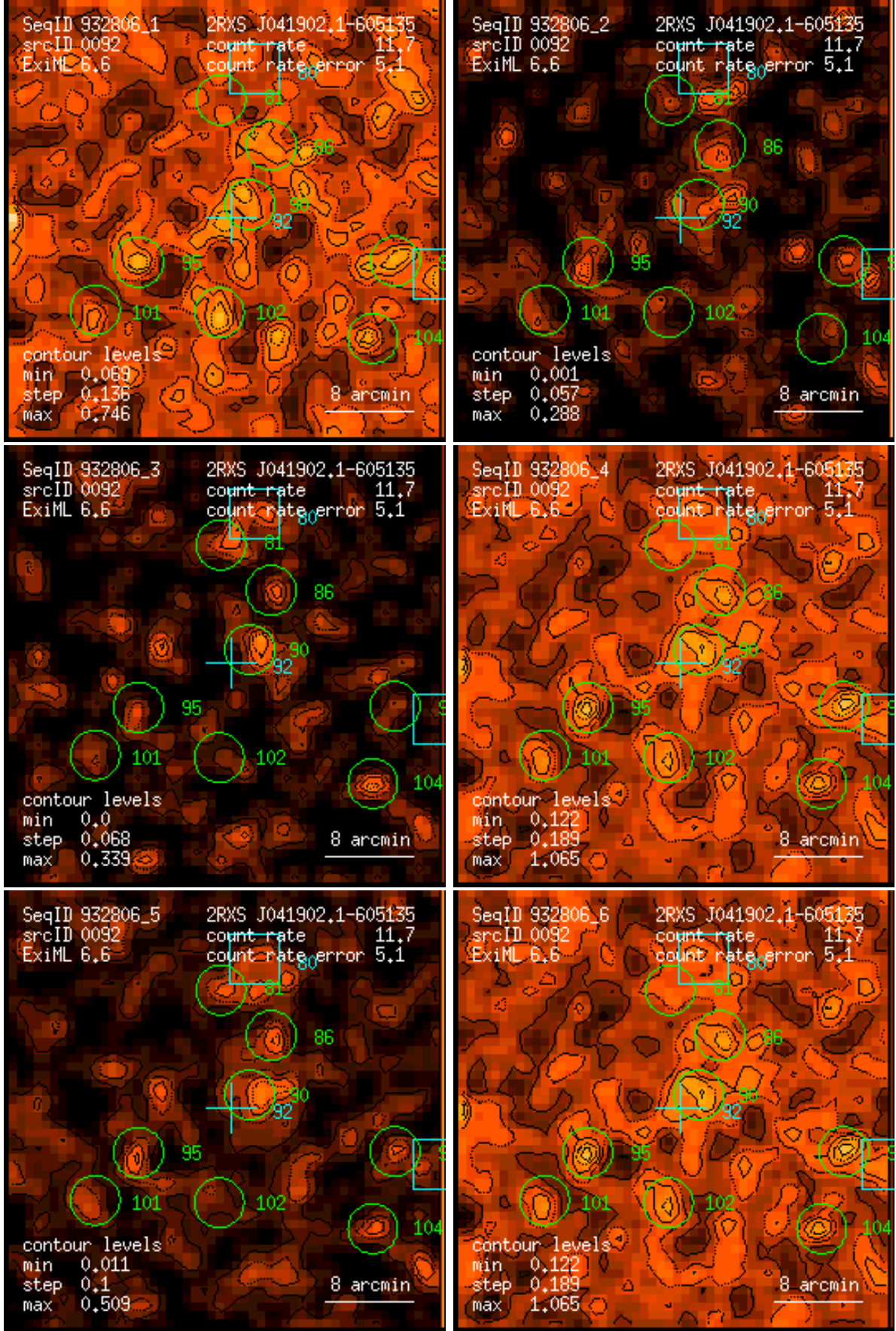
Figure 92: RASS 932806: detection 0092: band rate images, Gaussian filter: (1) PSPC channels 11 – 41, (2) 52 – 90, (3) 91 – 201, (4) 11 – 235, (5) 52 – 201, (6) 11 – 201. Broad band rates in counts/ks. Band rate contour levels in counts/ks/arcmin 2 .
