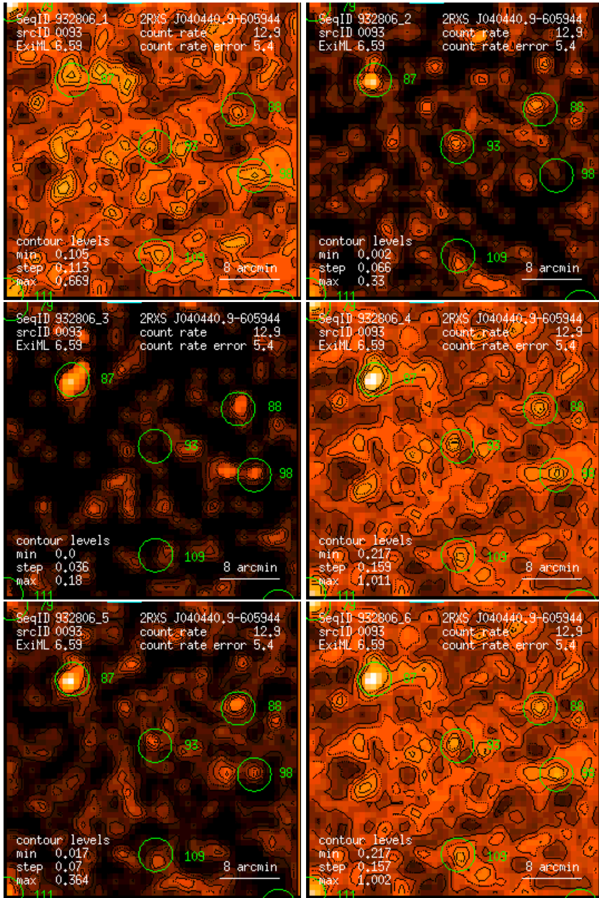
Figure 93: RASS 932806: detection 0093: band rate images, Gaussian filter: (1) PSPC channels 11 – 41, (2) 52 – 90, (3) 91 – 201, (4) 11 – 235, (5) 52 – 201, (6) 11 – 201. Broad band rates in counts/ks. Band rate contour levels in counts/ks/arcmin 2 .
