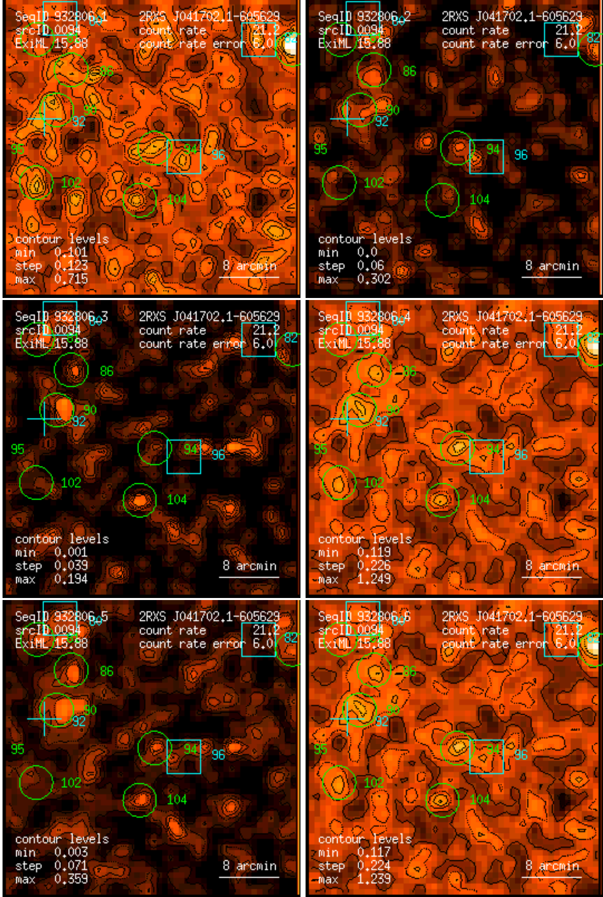
Figure 94: RASS 932806: detection 0094: band rate images, Gaussian filter: (1) PSPC channels 11 – 41, (2) 52 – 90, (3) 91 – 201, (4) 11 – 235, (5) 52 – 201, (6) 11 – 201. Broad band rates in counts/ks. Band rate contour levels in counts/ks/arcmin 2 .
