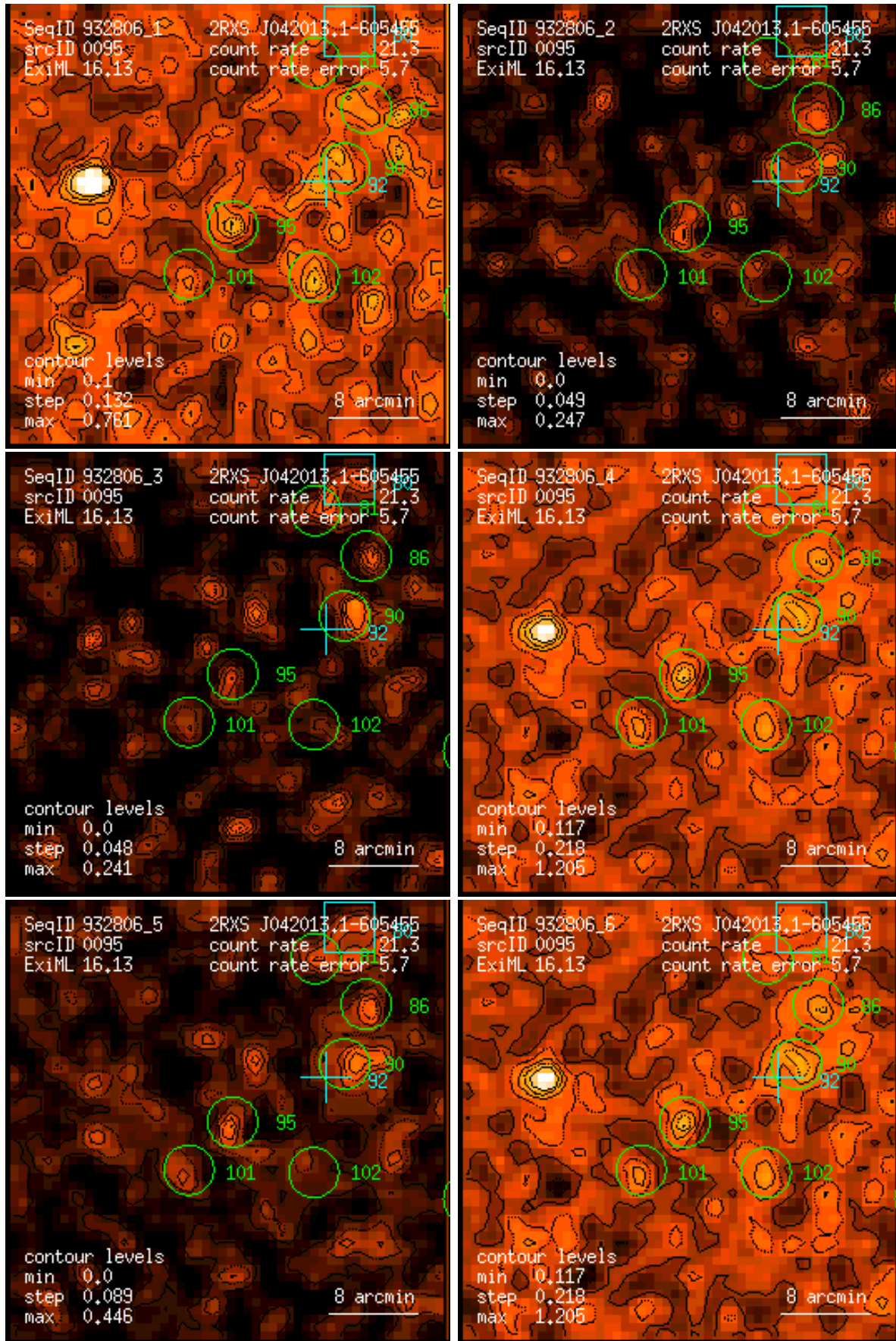
Figure 95: RASS 932806: detection 0095: band rate images, Gaussian filter: (1) PSPC channels 11 – 41, (2) 52 – 90, (3) 91 – 201, (4) 11 – 235, (5) 52 – 201, (6) 11 – 201. Broad band rates in counts/ks. Band rate contour levels in counts/ks/arcmin 2 .
