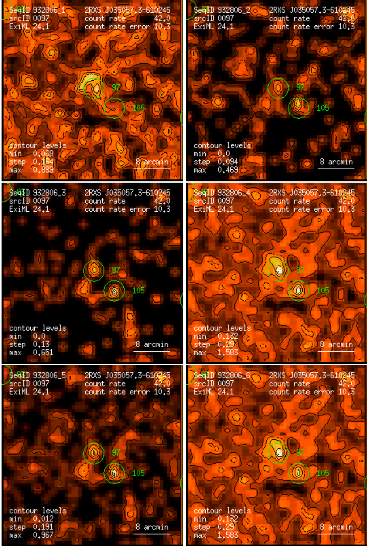
Figure 97: RASS 932806: detection 0097: band rate images, Gaussian filter: (1) PSPC channels 11 – 41, (2) 52 – 90, (3) 91 – 201, (4) 11 – 235, (5) 52 – 201, (6) 11 – 201. Broad band rates in counts/ks. Band rate contour levels in counts/ks/arcmin 2 .
