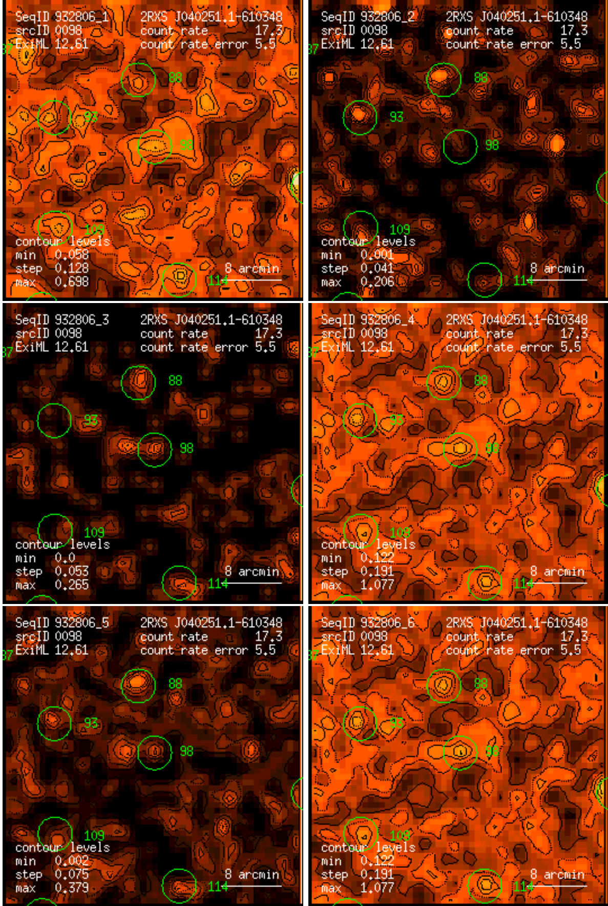
Figure 98: RASS 932806: detection 0098: band rate images, Gaussian filter: (1) PSPC channels 11 – 41, (2) 52 – 90, (3) 91 – 201, (4) 11 – 235, (5) 52 – 201, (6) 11 – 201. Broad band rates in counts/ks. Band rate contour levels in counts/ks/arcmin 2 .
