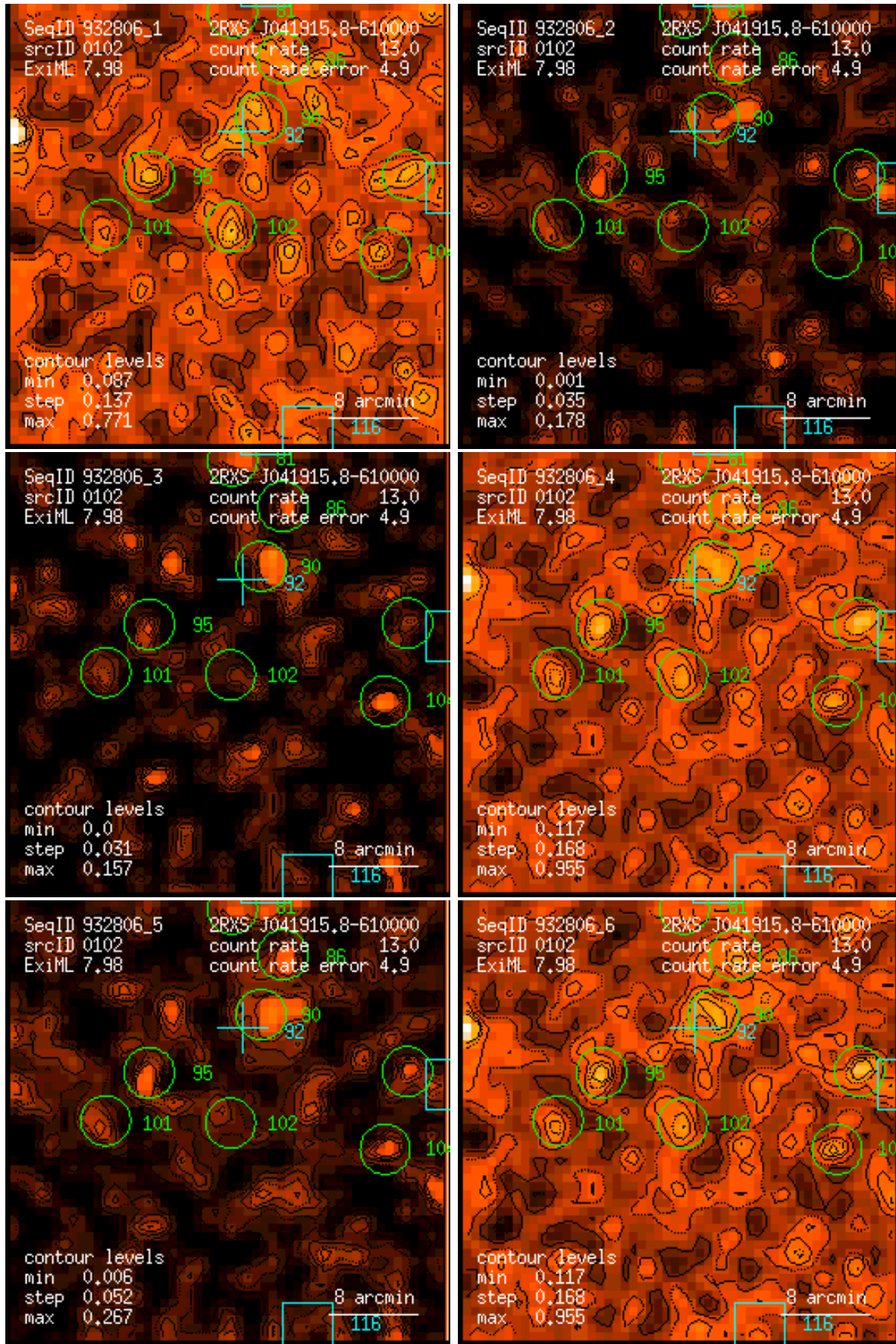
Figure 102: RASS 932806: detection 0102: band rate images, Gaussian filter: (1) PSPC channels 11 – 41, (2) 52 – 90, (3) 91 – 201, (4) 11 – 235, (5) 52 – 201, (6) 11 – 201. Broad band rates in counts/ks. Band rate contour levels in counts/ks/arcmin 2 .
