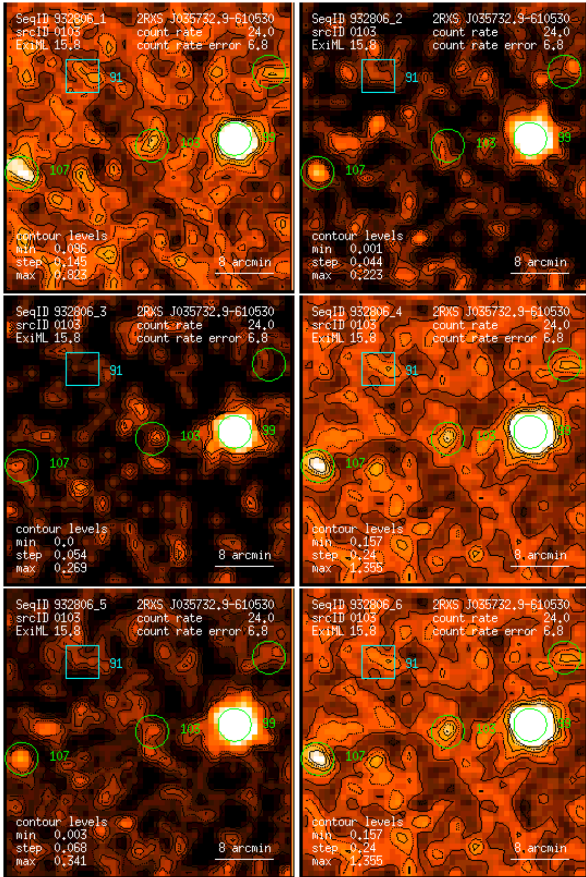
Figure 103: RASS 932806: detection 0103: band rate images, Gaussian filter: (1) PSPC channels 11 – 41, (2) 52 – 90, (3) 91 – 201, (4) 11 – 235, (5) 52 – 201, (6) 11 – 201. Broad band rates in counts/ks. Band rate contour levels in counts/ks/arcmin 2 .
