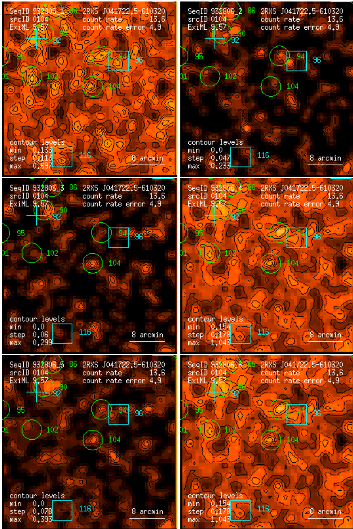
Figure 104: RASS 932806: detection 0104: band rate images, Gaussian filter: (1) PSPC channels 11 – 41, (2) 52 – 90, (3) 91 – 201, (4) 11 – 235, (5) 52 – 201, (6) 11 – 201. Broad band rates in counts/ks. Band rate contour levels in counts/ks/arcmin 2 .
