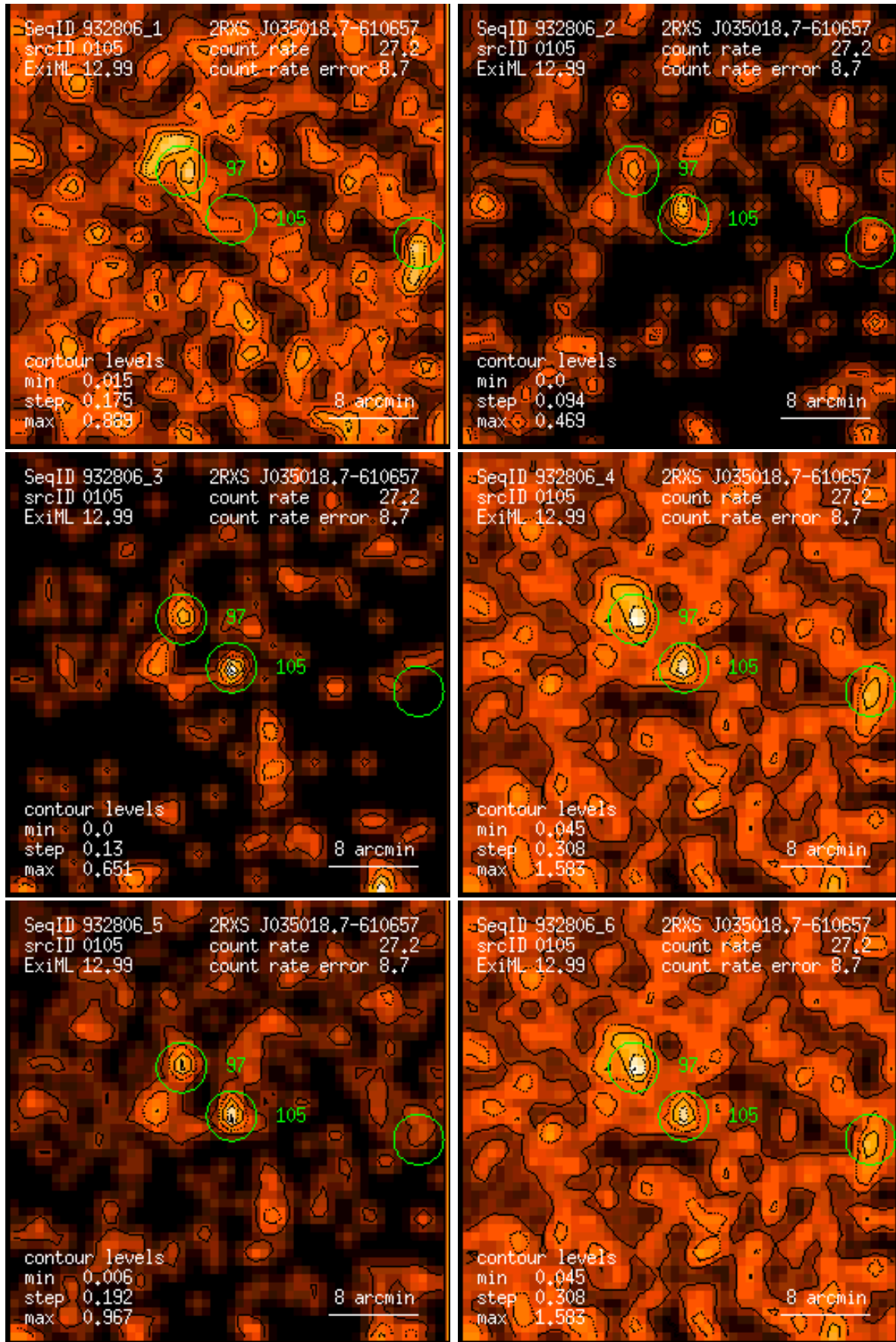
Figure 105: RASS 932806: detection 0105: band rate images, Gaussian filter: (1) PSPC channels 11 – 41, (2) 52 – 90, (3) 91 – 201, (4) 11 – 235, (5) 52 – 201, (6) 11 – 201. Broad band rates in counts/ks. Band rate contour levels in counts/ks/arcmin 2 .
