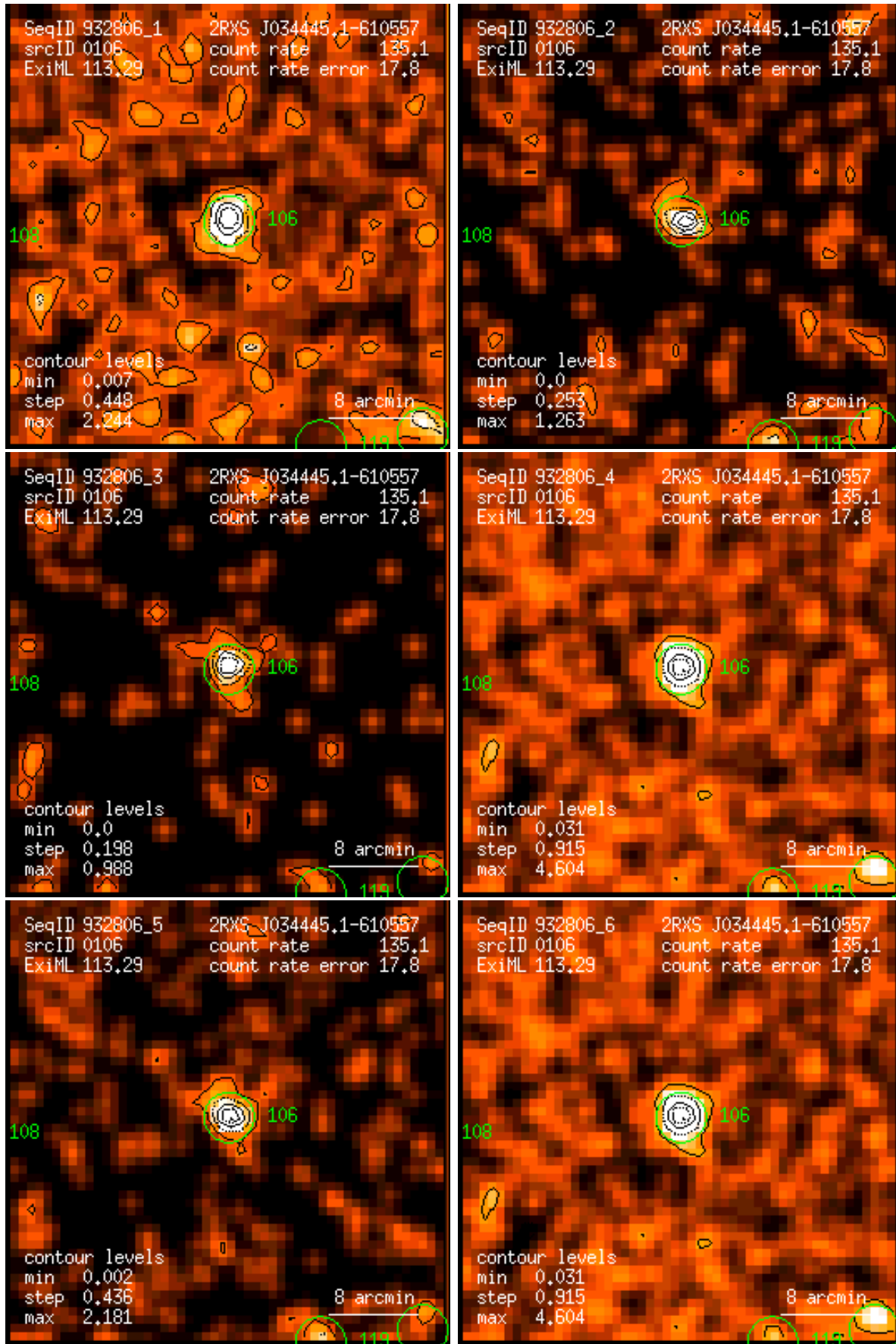
Figure 106: RASS 932806: detection 0106: band rate images, Gaussian filter: (1) PSPC channels 11 – 41, (2) 52 – 90, (3) 91 – 201, (4) 11 – 235, (5) 52 – 201, (6) 11 – 201. Broad band rates in counts/ks. Band rate contour levels in counts/ks/arcmin 2 .
