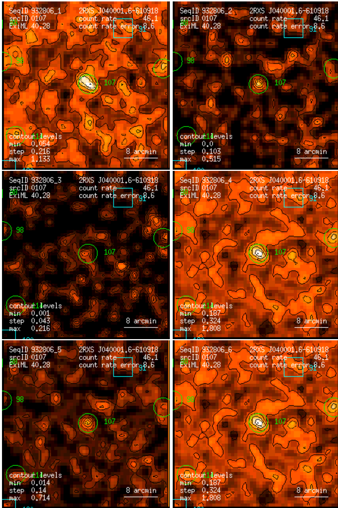
Figure 107: RASS 932806: detection 0107: band rate images, Gaussian filter: (1) PSPC channels 11 – 41, (2) 52 – 90, (3) 91 – 201, (4) 11 – 235, (5) 52 – 201, (6) 11 – 201. Broad band rates in counts/ks. Band rate contour levels in counts/ks/arcmin 2 .
