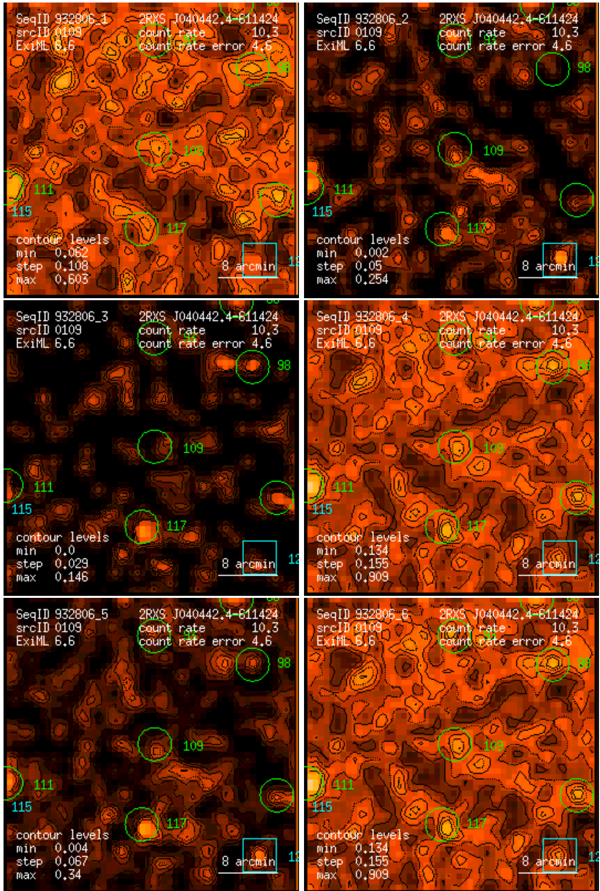
Figure 109: RASS 932806: detection 0109: band rate images, Gaussian filter: (1) PSPC channels 11 – 41, (2) 52 – 90, (3) 91 – 201, (4) 11 – 235, (5) 52 – 201, (6) 11 – 201. Broad band rates in counts/ks. Band rate contour levels in counts/ks/arcmin 2 .
