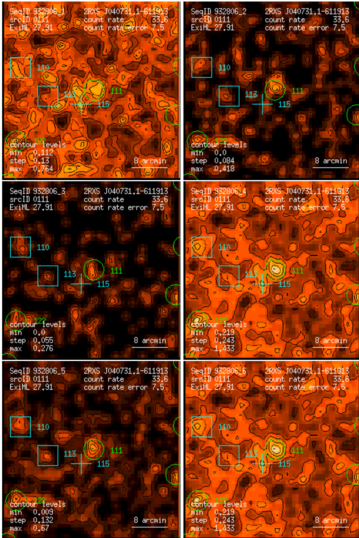
Figure 111: RASS 932806: detection 0111: band rate images, Gaussian filter: (1) PSPC channels 11 – 41, (2) 52 – 90, (3) 91 – 201, (4) 11 – 235, (5) 52 – 201, (6) 11 – 201. Broad band rates in counts/ks. Band rate contour levels in counts/ks/arcmin 2 .
