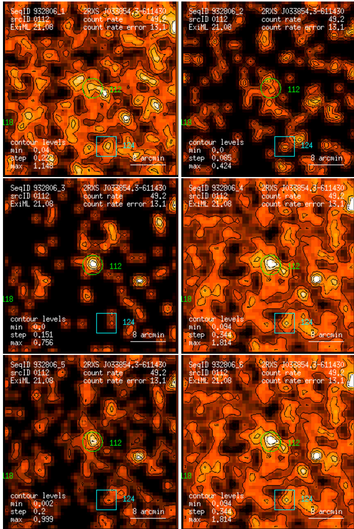
Figure 112: RASS 932806: detection 0112: band rate images, Gaussian filter: (1) PSPC channels 11 – 41, (2) 52 – 90, (3) 91 – 201, (4) 11 – 235, (5) 52 – 201, (6) 11 – 201. Broad band rates in counts/ks. Band rate contour levels in counts/ks/arcmin 2 .
