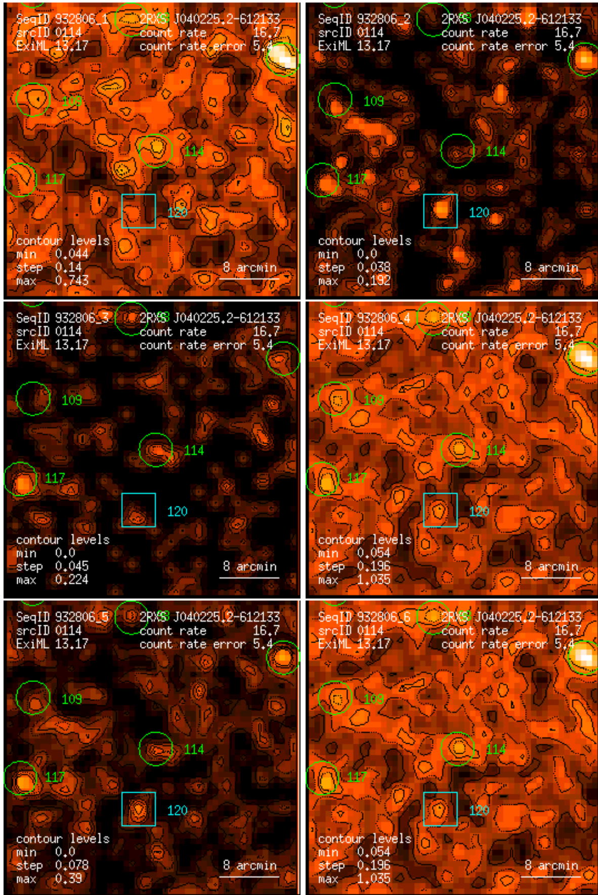
Figure 114: RASS 932806: detection 0114: band rate images, Gaussian filter: (1) PSPC channels 11 – 41, (2) 52 – 90, (3) 91 – 201, (4) 11 – 235, (5) 52 – 201, (6) 11 – 201. Broad band rates in counts/ks. Band rate contour levels in counts/ks/arcmin 2 .
