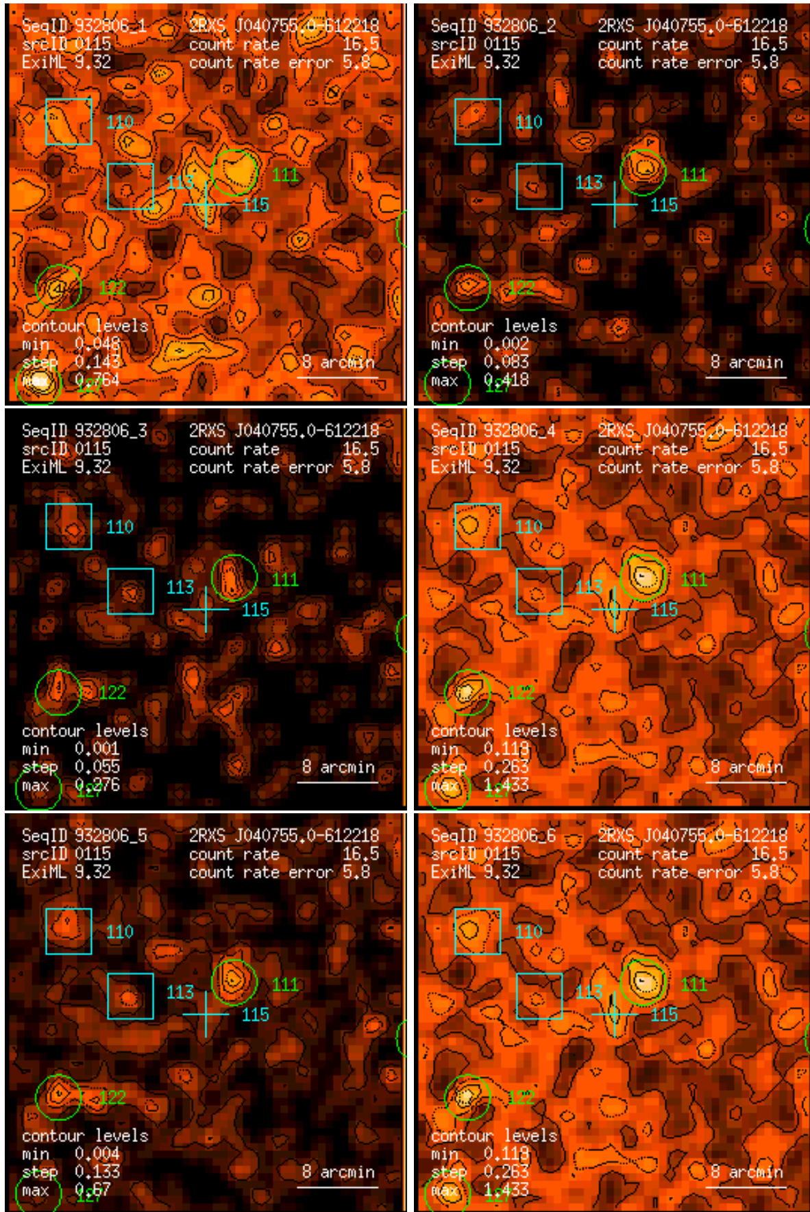
Figure 115: RASS 932806: detection 0115: band rate images, Gaussian filter: (1) PSPC channels 11 – 41, (2) 52 – 90, (3) 91 – 201, (4) 11 – 235, (5) 52 – 201, (6) 11 – 201. Broad band rates in counts/ks. Band rate contour levels in counts/ks/arcmin 2 .
