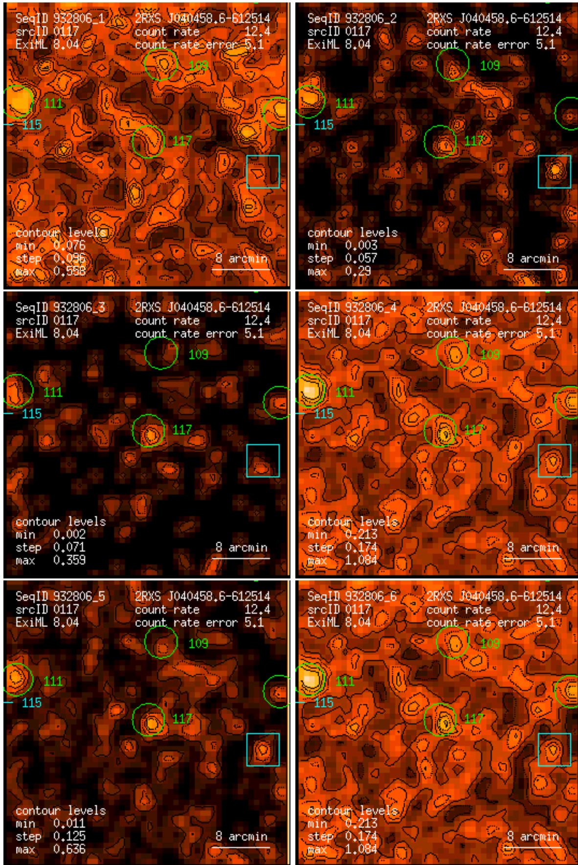
Figure 117: RASS 932806: detection 0117: band rate images, Gaussian filter: (1) PSPC channels 11 – 41, (2) 52 – 90, (3) 91 – 201, (4) 11 – 235, (5) 52 – 201, (6) 11 – 201. Broad band rates in counts/ks. Band rate contour levels in counts/ks/arcmin 2 .
