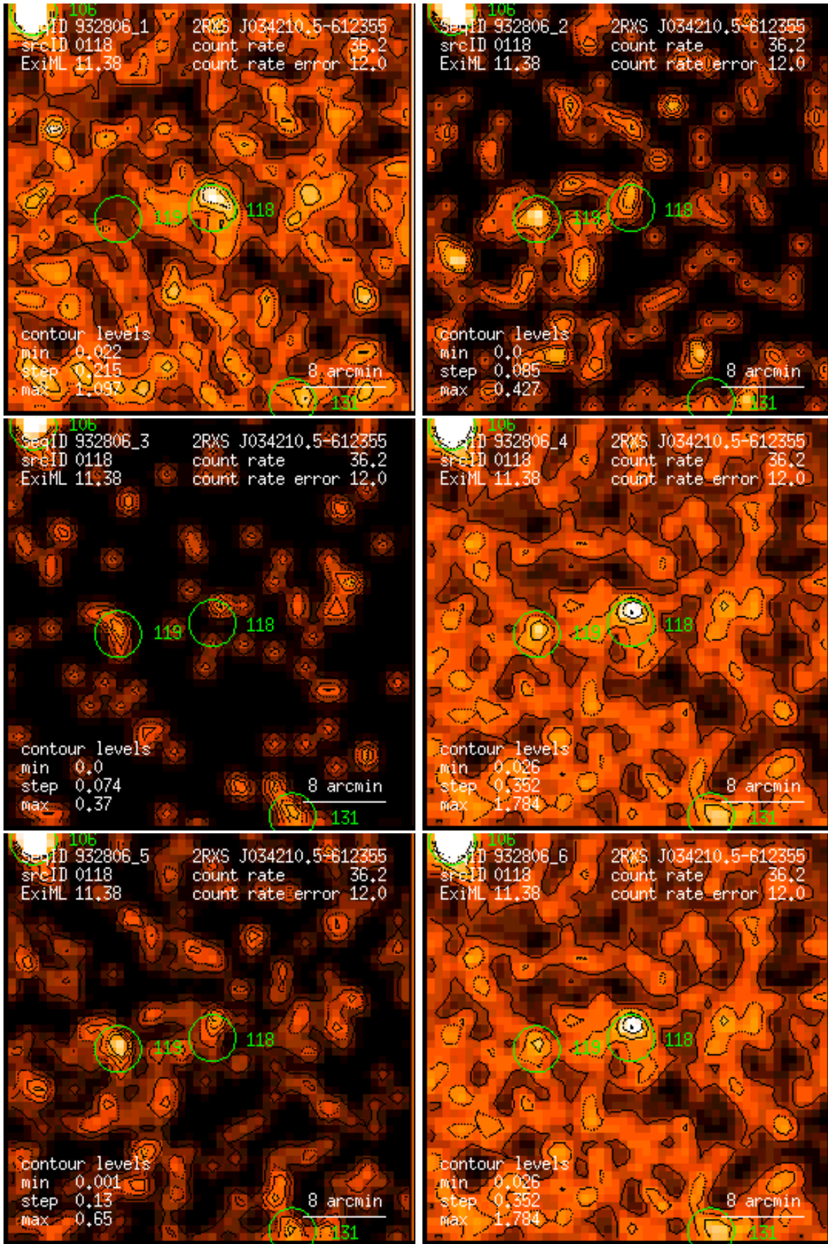
Figure 118: RASS 932806: detection 0118: band rate images, Gaussian filter: (1) PSPC channels 11 – 41, (2) 52 – 90, (3) 91 – 201, (4) 11 – 235, (5) 52 – 201, (6) 11 – 201. Broad band rates in counts/ks. Band rate contour levels in counts/ks/arcmin 2 .
