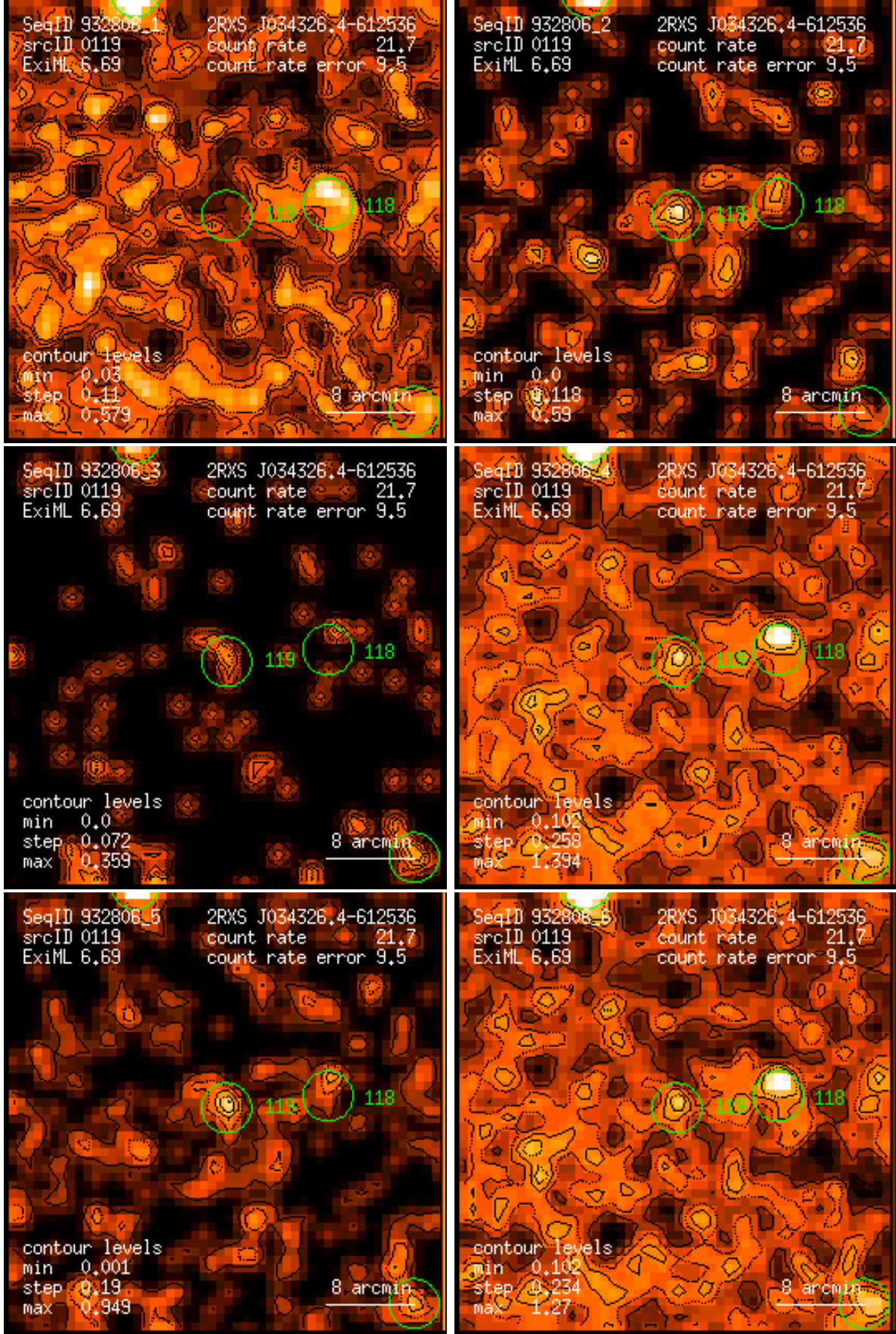
Figure 119: RASS 932806: detection 0119: band rate images, Gaussian filter: (1) PSPC channels 11 – 41, (2) 52 – 90, (3) 91 – 201, (4) 11 – 235, (5) 52 – 201, (6) 11 – 201. Broad band rates in counts/ks. Band rate contour levels in counts/ks/arcmin 2 .
