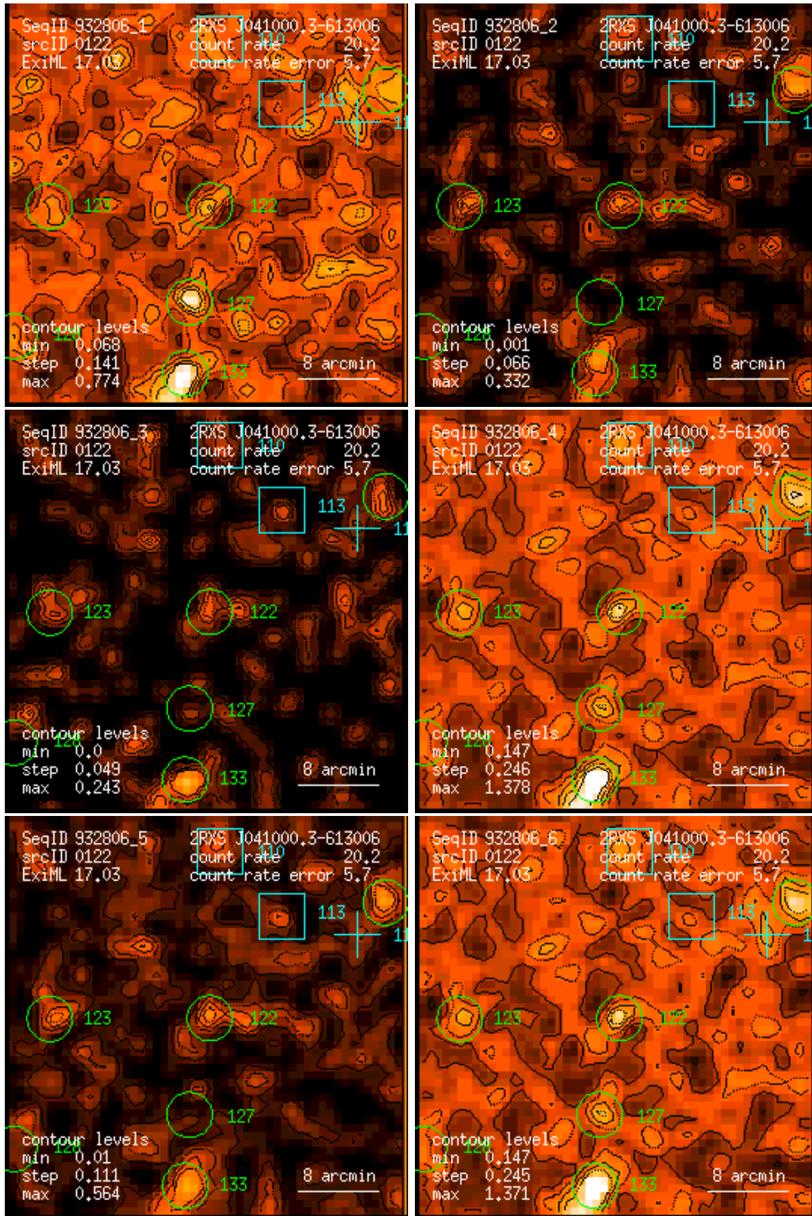
Figure 122: RASS 932806: detection 0122: band rate images, Gaussian filter: (1) PSPC channels 11 – 41, (2) 52 – 90, (3) 91 – 201, (4) 11 – 235, (5) 52 – 201, (6) 11 – 201. Broad band rates in counts/ks. Band rate contour levels in counts/ks/arcmin 2 .
