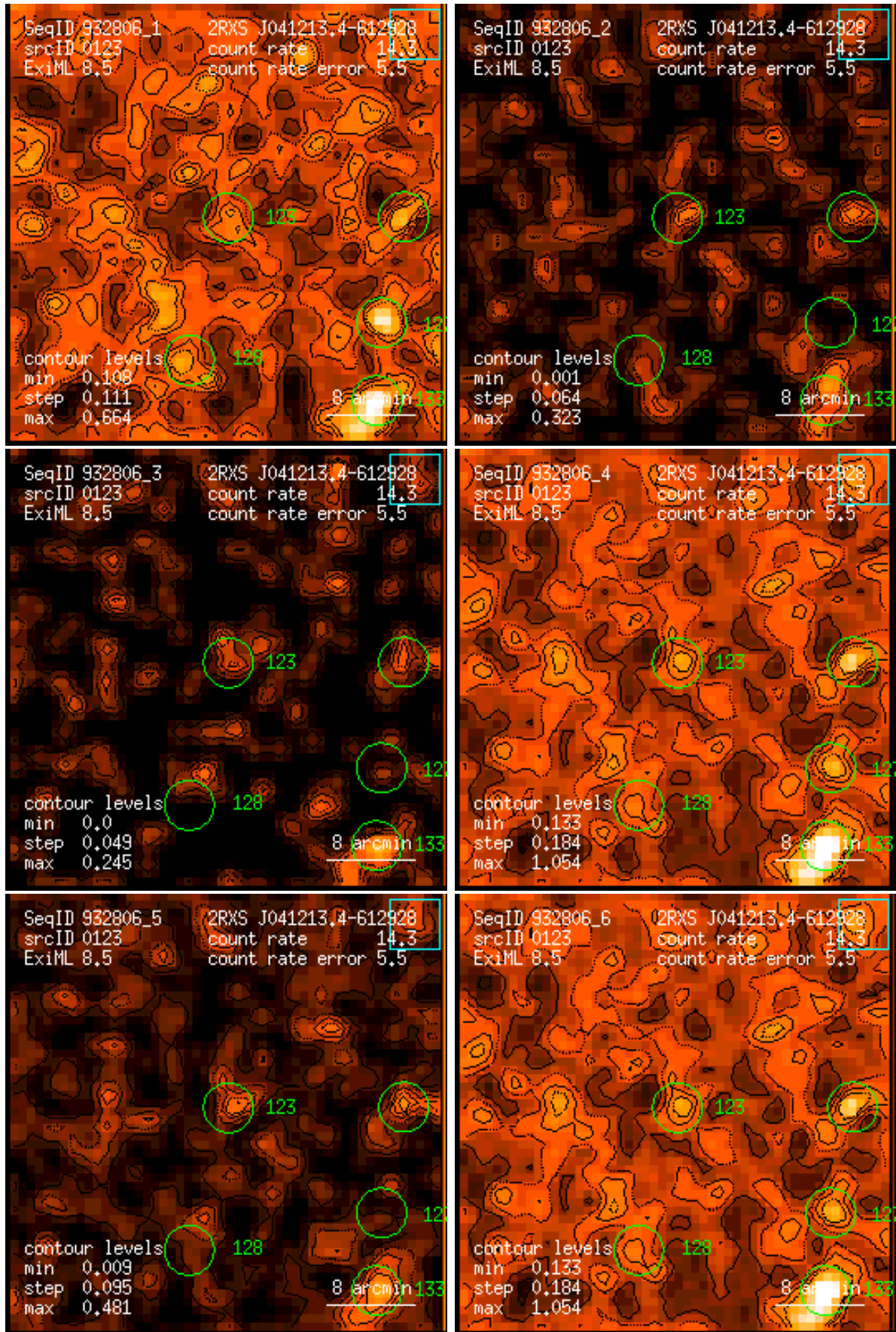
Figure 123: RASS 932806: detection 0123: band rate images, Gaussian filter: (1) PSPC channels 11 – 41, (2) 52 – 90, (3) 91 – 201, (4) 11 – 235, (5) 52 – 201, (6) 11 – 201. Broad band rates in counts/ks. Band rate contour levels in counts/ks/arcmin 2 .
