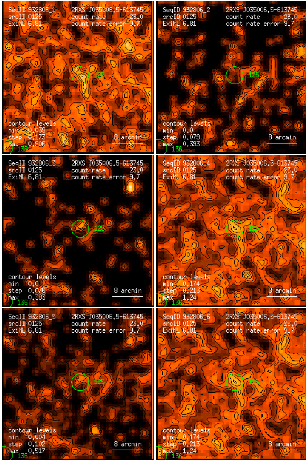
Figure 125: RASS 932806: detection 0125: band rate images, Gaussian filter: (1) PSPC channels 11 – 41, (2) 52 – 90, (3) 91 – 201, (4) 11 – 235, (5) 52 – 201, (6) 11 – 201. Broad band rates in counts/ks. Band rate contour levels in counts/ks/arcmin 2 .
