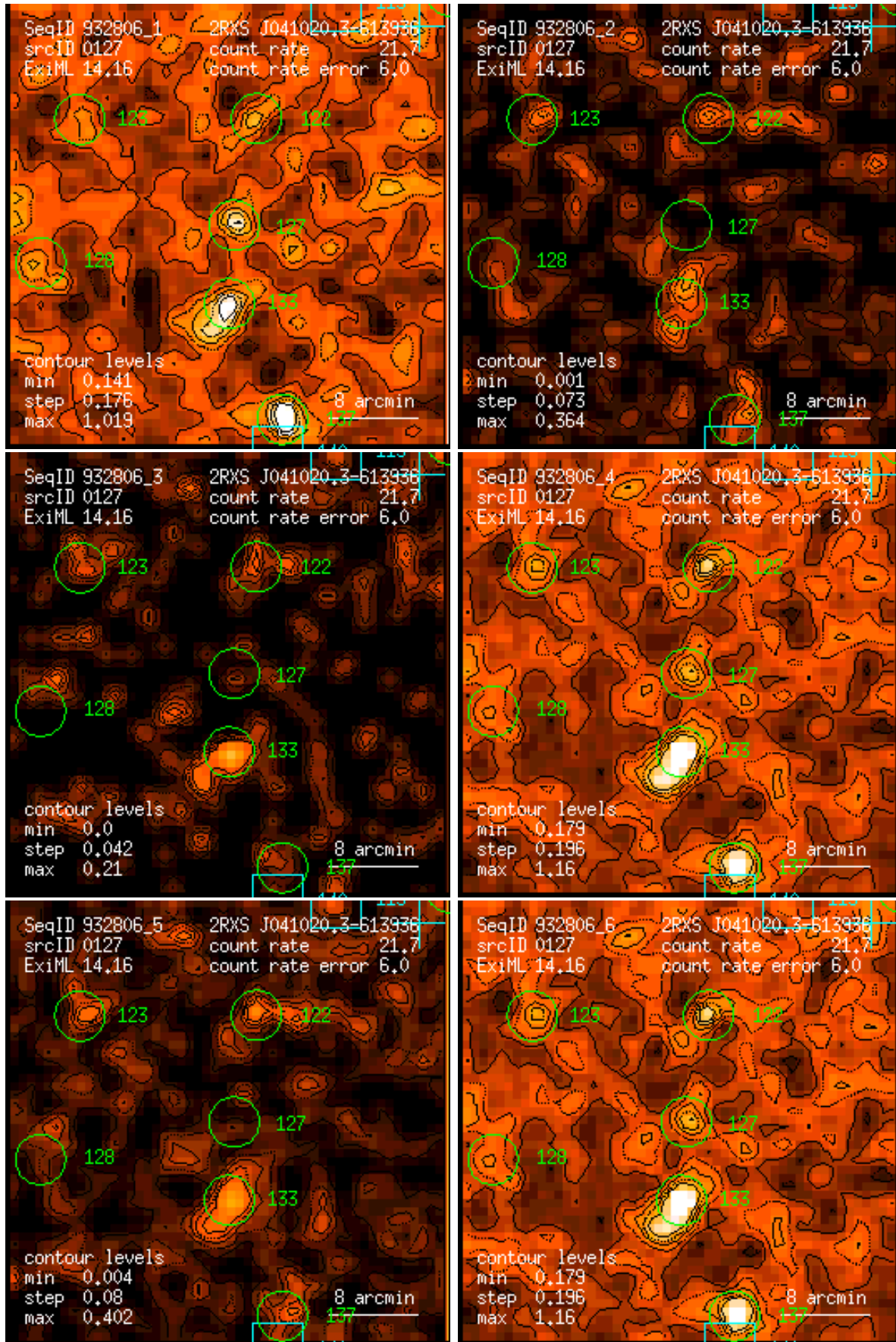
Figure 127: RASS 932806: detection 0127: band rate images, Gaussian filter: (1) PSPC channels 11 – 41, (2) 52 – 90, (3) 91 – 201, (4) 11 – 235, (5) 52 – 201, (6) 11 – 201. Broad band rates in counts/ks. Band rate contour levels in counts/ks/arcmin 2 .
