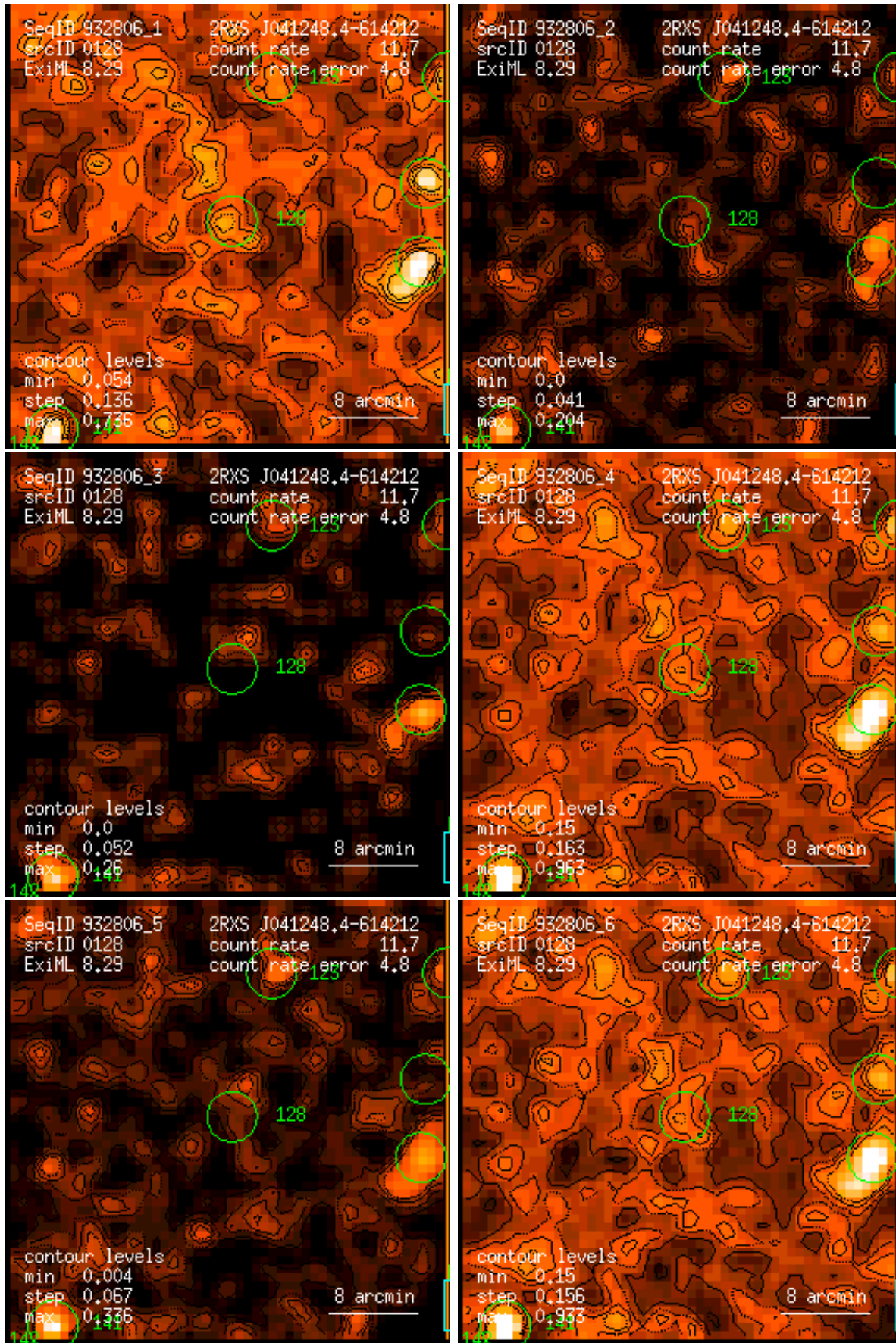
Figure 128: RASS 932806: detection 0128: band rate images, Gaussian filter: (1) PSPC channels 11 – 41, (2) 52 – 90, (3) 91 – 201, (4) 11 – 235, (5) 52 – 201, (6) 11 – 201. Broad band rates in counts/ks. Band rate contour levels in counts/ks/arcmin 2 .
