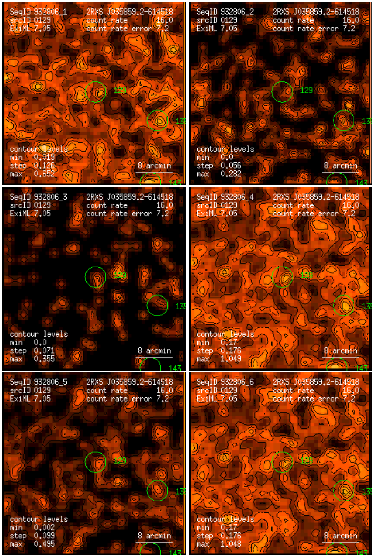
Figure 129: RASS 932806: detection 0129: band rate images, Gaussian filter: (1) PSPC channels 11 – 41, (2) 52 – 90, (3) 91 – 201, (4) 11 – 235, (5) 52 – 201, (6) 11 – 201. Broad band rates in counts/ks. Band rate contour levels in counts/ks/arcmin 2 .
