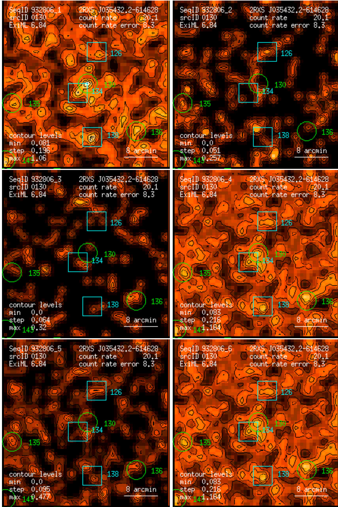
Figure 130: RASS 932806: detection 0130: band rate images, Gaussian filter: (1) PSPC channels 11 – 41, (2) 52 – 90, (3) 91 – 201, (4) 11 – 235, (5) 52 – 201, (6) 11 – 201. Broad band rates in counts/ks. Band rate contour levels in counts/ks/arcmin 2 .
