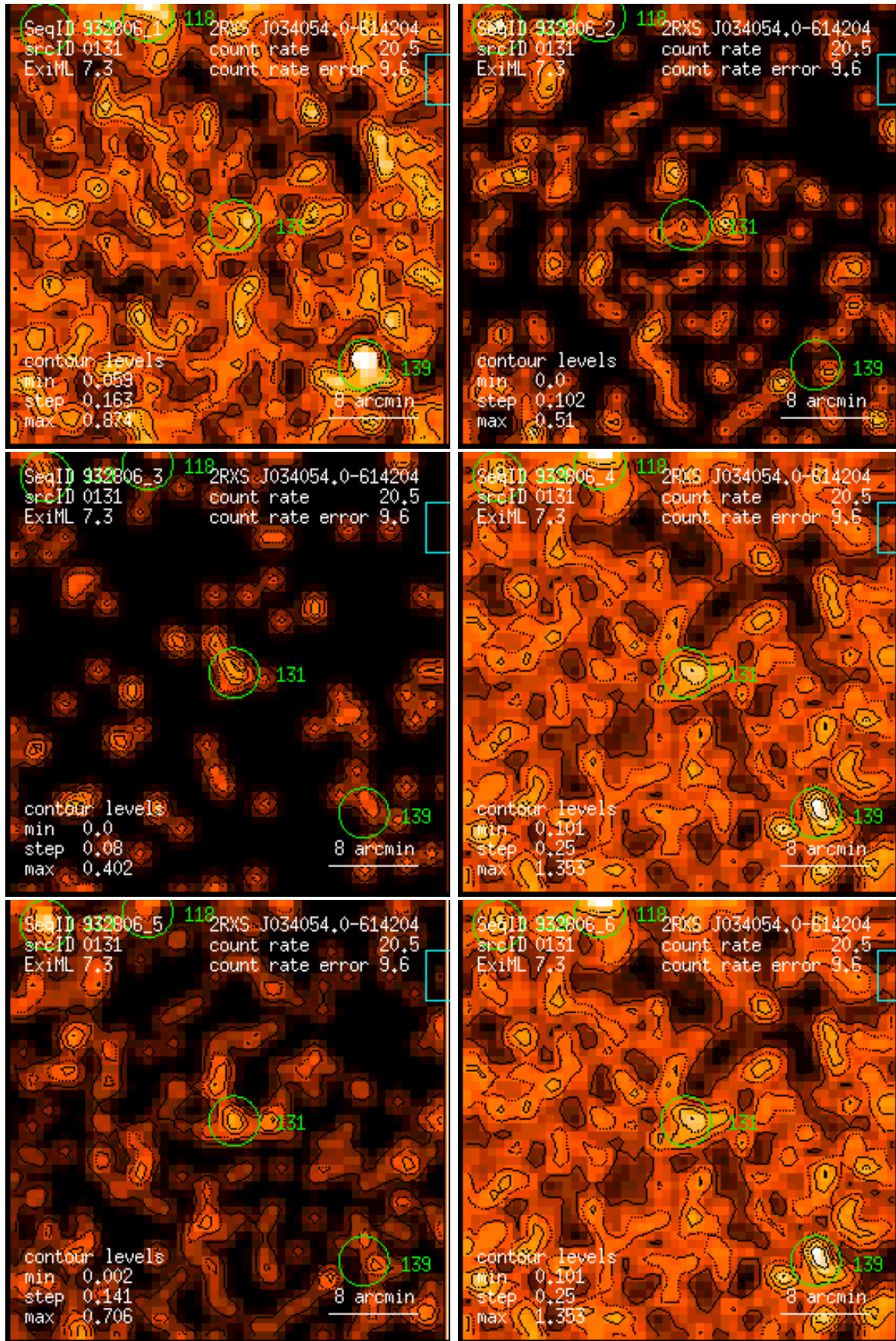
Figure 131: RASS 932806: detection 0131: band rate images, Gaussian filter: (1) PSPC channels 11 – 41, (2) 52 – 90, (3) 91 – 201, (4) 11 – 235, (5) 52 – 201, (6) 11 – 201. Broad band rates in counts/ks. Band rate contour levels in counts/ks/arcmin 2 .
