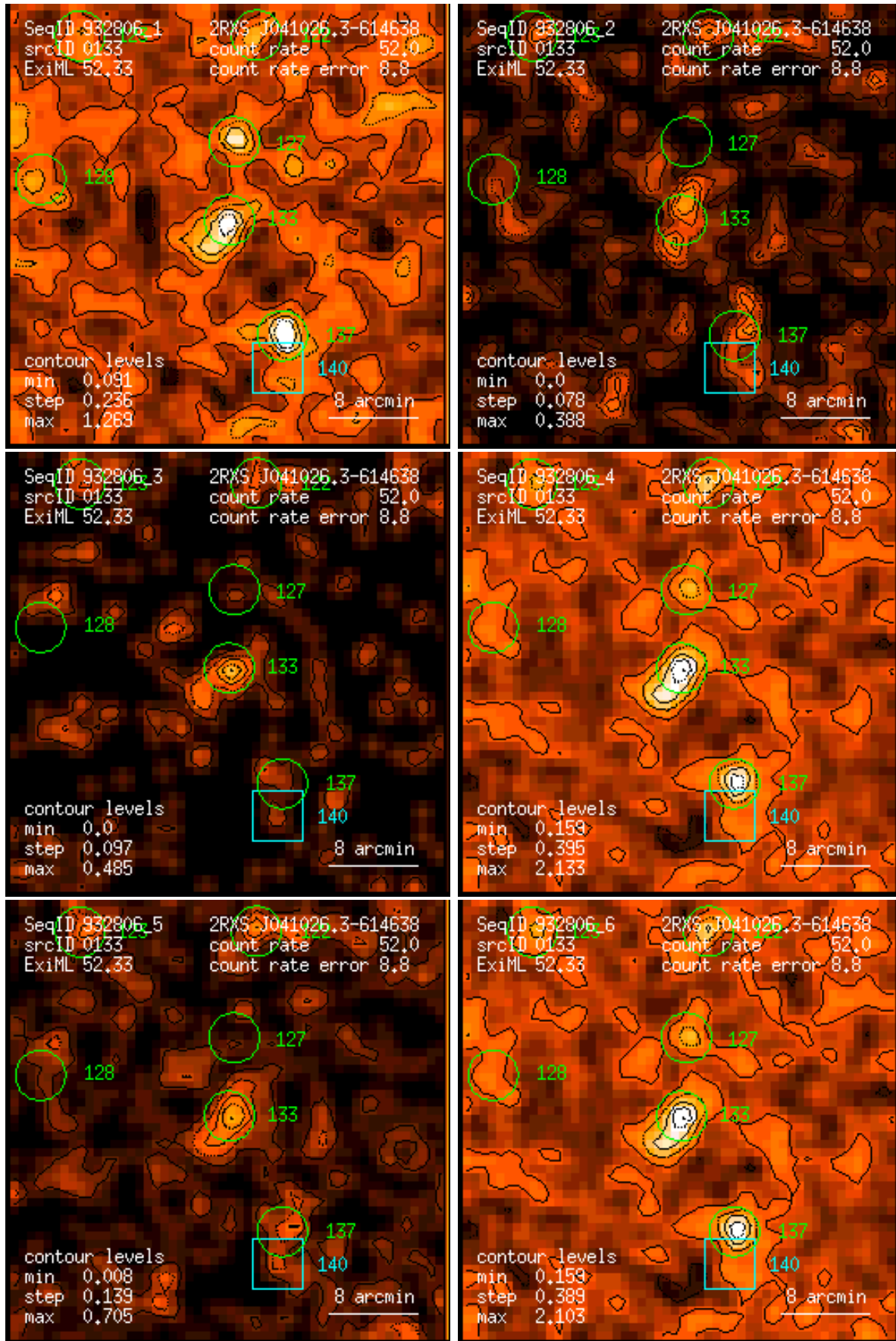
Figure 133: RASS 932806: detection 0133: band rate images, Gaussian filter: (1) PSPC channels 11 – 41, (2) 52 – 90, (3) 91 – 201, (4) 11 – 235, (5) 52 – 201, (6) 11 – 201. Broad band rates in counts/ks. Band rate contour levels in counts/ks/arcmin 2 .
