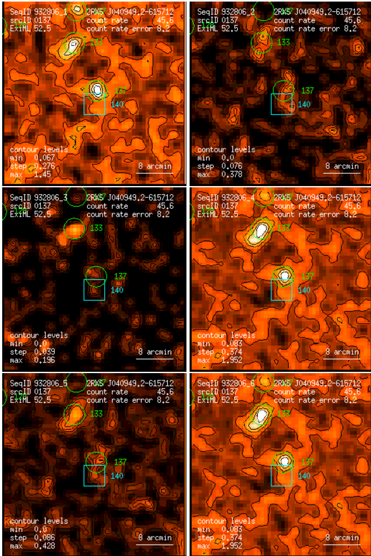
Figure 137: RASS 932806: detection 0137: band rate images, Gaussian filter: (1) PSPC channels 11 – 41, (2) 52 – 90, (3) 91 – 201, (4) 11 – 235, (5) 52 – 201, (6) 11 – 201. Broad band rates in counts/ks. Band rate contour levels in counts/ks/arcmin 2 .
