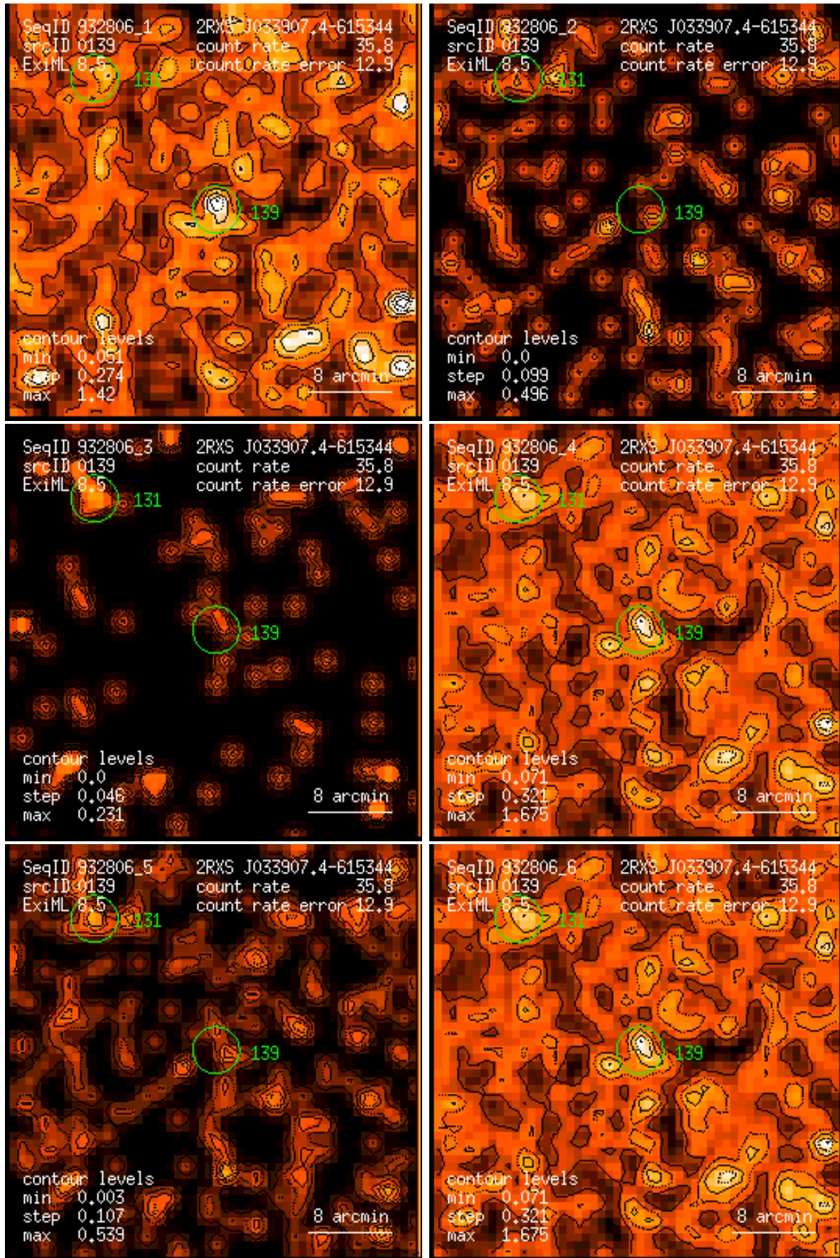
Figure 139: RASS 932806: detection 0139: band rate images, Gaussian filter: (1) PSPC channels 11 – 41, (2) 52 – 90, (3) 91 – 201, (4) 11 – 235, (5) 52 – 201, (6) 11 – 201. Broad band rates in counts/ks. Band rate contour levels in counts/ks/arcmin 2 .
