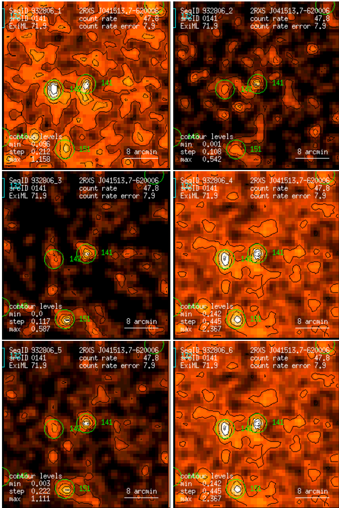
Figure 141: RASS 932806: detection 0141: band rate images, Gaussian filter: (1) PSPC channels 11 – 41, (2) 52 – 90, (3) 91 – 201, (4) 11 – 235, (5) 52 – 201, (6) 11 – 201. Broad band rates in counts/ks. Band rate contour levels in counts/ks/arcmin 2 .
