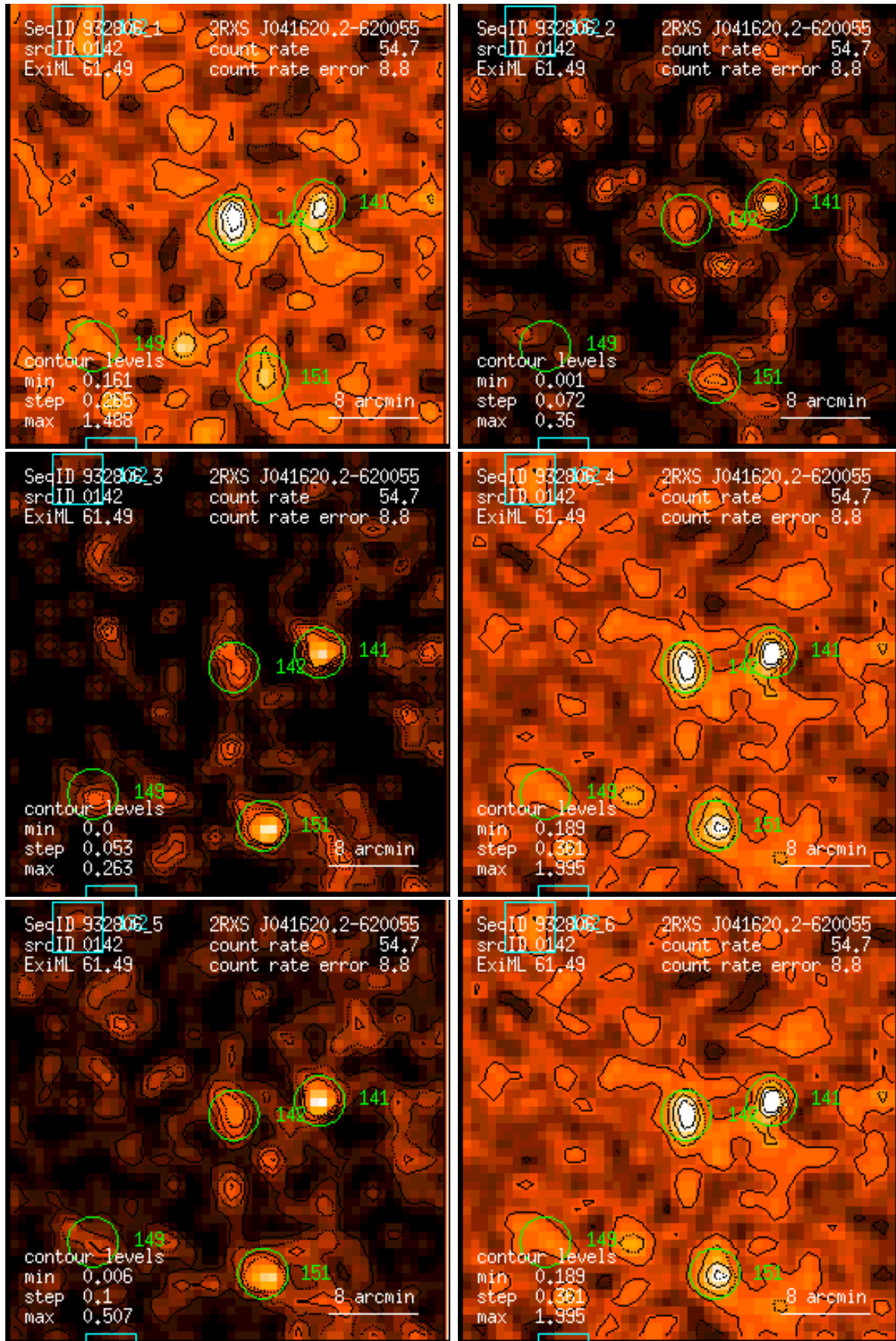
Figure 142: RASS 932806: detection 0142: band rate images, Gaussian filter: (1) PSPC channels 11 – 41, (2) 52 – 90, (3) 91 – 201, (4) 11 – 235, (5) 52 – 201, (6) 11 – 201. Broad band rates in counts/ks. Band rate contour levels in counts/ks/arcmin 2 .
