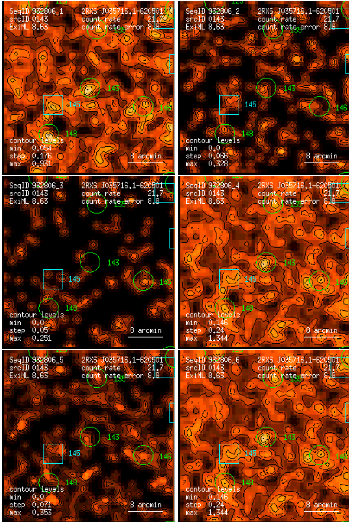
Figure 143: RASS 932806: detection 0143: band rate images, Gaussian filter: (1) PSPC channels 11 – 41, (2) 52 – 90, (3) 91 – 201, (4) 11 – 235, (5) 52 – 201, (6) 11 – 201. Broad band rates in counts/ks. Band rate contour levels in counts/ks/arcmin 2 .
