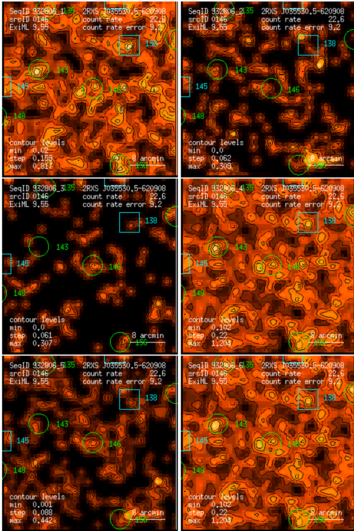
Figure 146: RASS 932806: detection 0146: band rate images, Gaussian filter: (1) PSPC channels 11 – 41, (2) 52 – 90, (3) 91 – 201, (4) 11 – 235, (5) 52 – 201, (6) 11 – 201. Broad band rates in counts/ks. Band rate contour levels in counts/ks/arcmin 2 .
