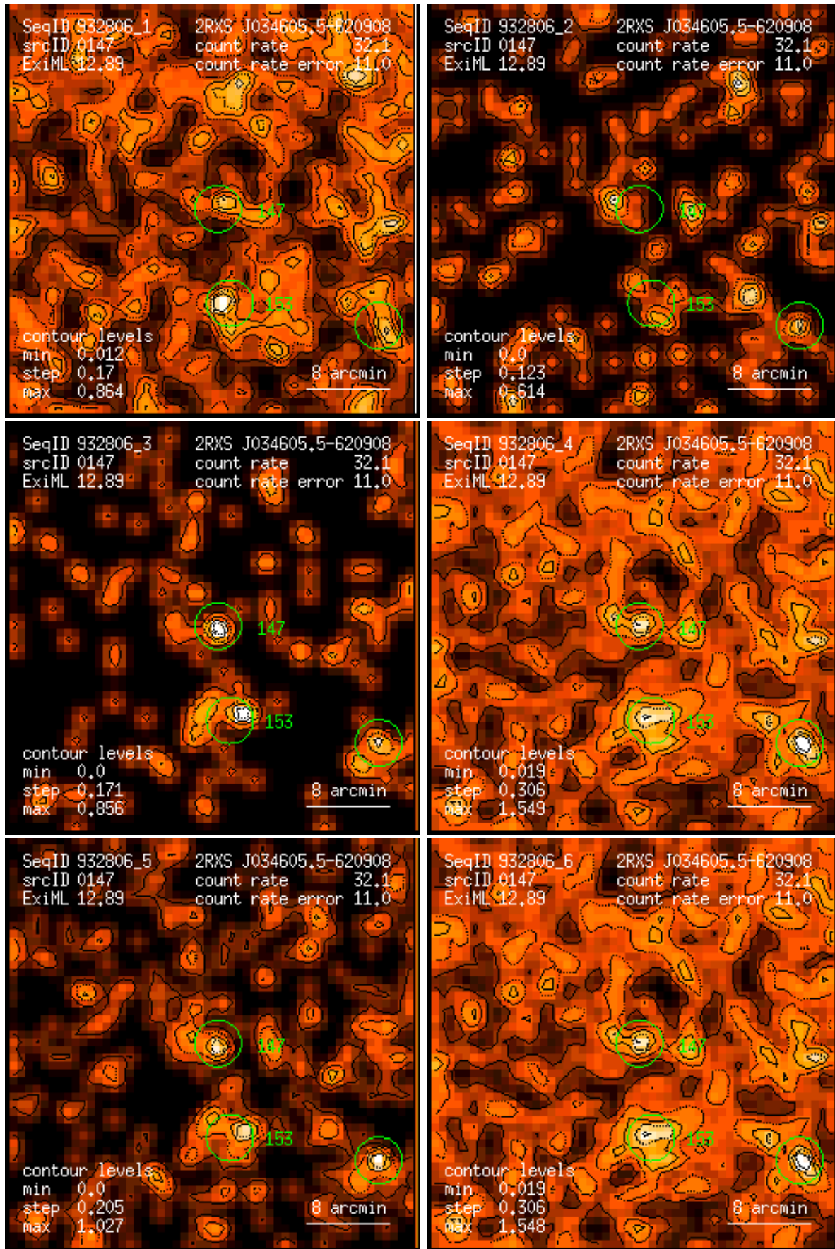
Figure 147: RASS 932806: detection 0147: band rate images, Gaussian filter: (1) PSPC channels 11 – 41, (2) 52 – 90, (3) 91 – 201, (4) 11 – 235, (5) 52 – 201, (6) 11 – 201. Broad band rates in counts/ks. Band rate contour levels in counts/ks/arcmin 2 .
