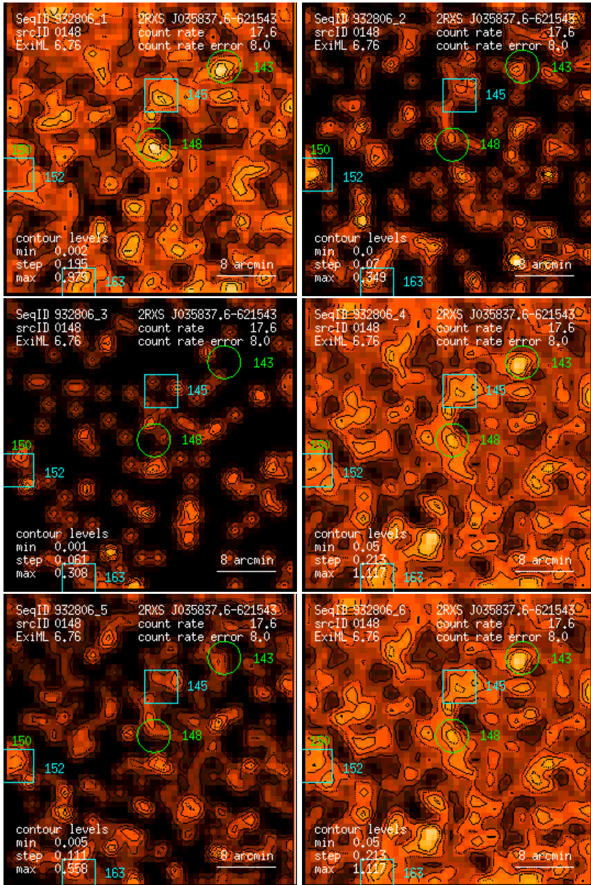
Figure 148: RASS 932806: detection 0148: band rate images, Gaussian filter: (1) PSPC channels 11 – 41, (2) 52 – 90, (3) 91 – 201, (4) 11 – 235, (5) 52 – 201, (6) 11 – 201. Broad band rates in counts/ks. Band rate contour levels in counts/ks/arcmin 2 .
