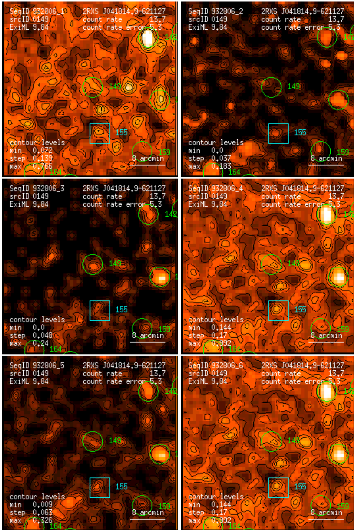
Figure 149: RASS 932806: detection 0149: band rate images, Gaussian filter: (1) PSPC channels 11 – 41, (2) 52 – 90, (3) 91 – 201, (4) 11 – 235, (5) 52 – 201, (6) 11 – 201. Broad band rates in counts/ks. Band rate contour levels in counts/ks/arcmin 2 .
