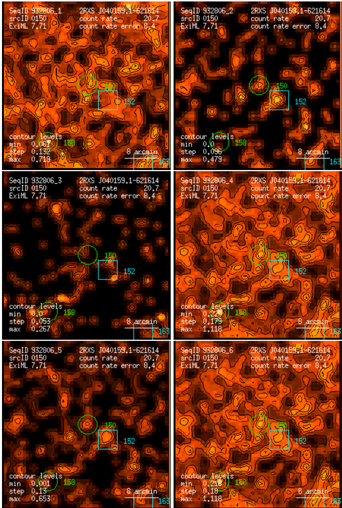
Figure 150: RASS 932806: detection 0150: band rate images, Gaussian filter: (1) PSPC channels 11 – 41, (2) 52 – 90, (3) 91 – 201, (4) 11 – 235, (5) 52 – 201, (6) 11 – 201. Broad band rates in counts/ks. Band rate contour levels in counts/ks/arcmin 2 .
