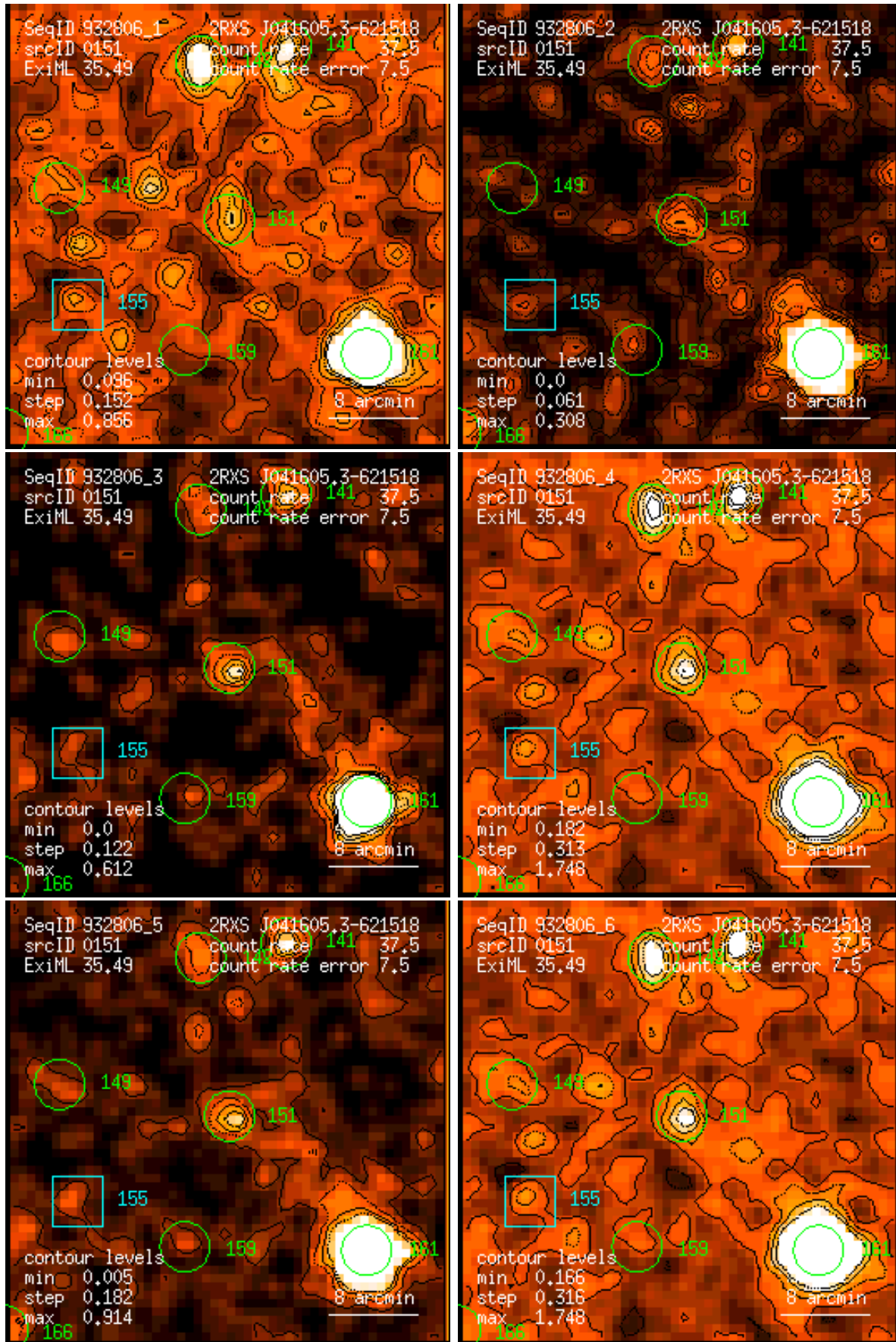
Figure 151: RASS 932806: detection 0151: band rate images, Gaussian filter: (1) PSPC channels 11 – 41, (2) 52 – 90, (3) 91 – 201, (4) 11 – 235, (5) 52 – 201, (6) 11 – 201. Broad band rates in counts/ks. Band rate contour levels in counts/ks/arcmin 2 .
